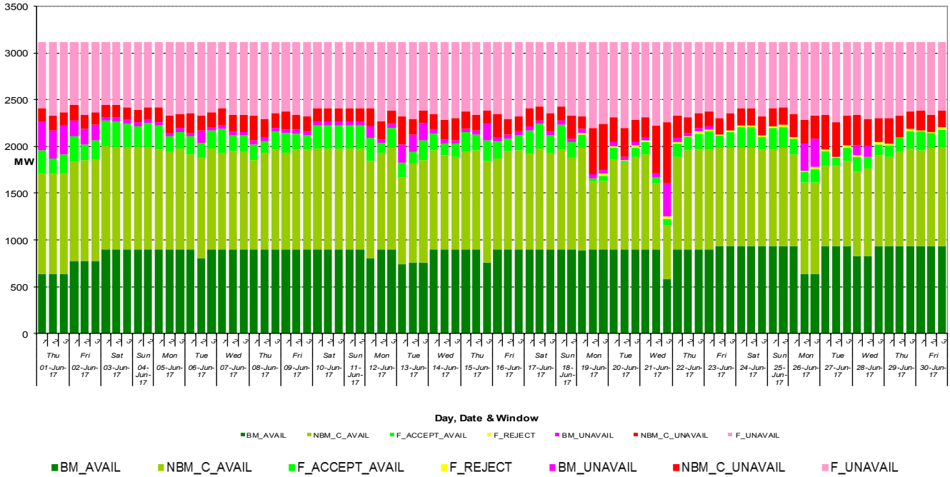
STOR MW Profile for month of Jun 2017
