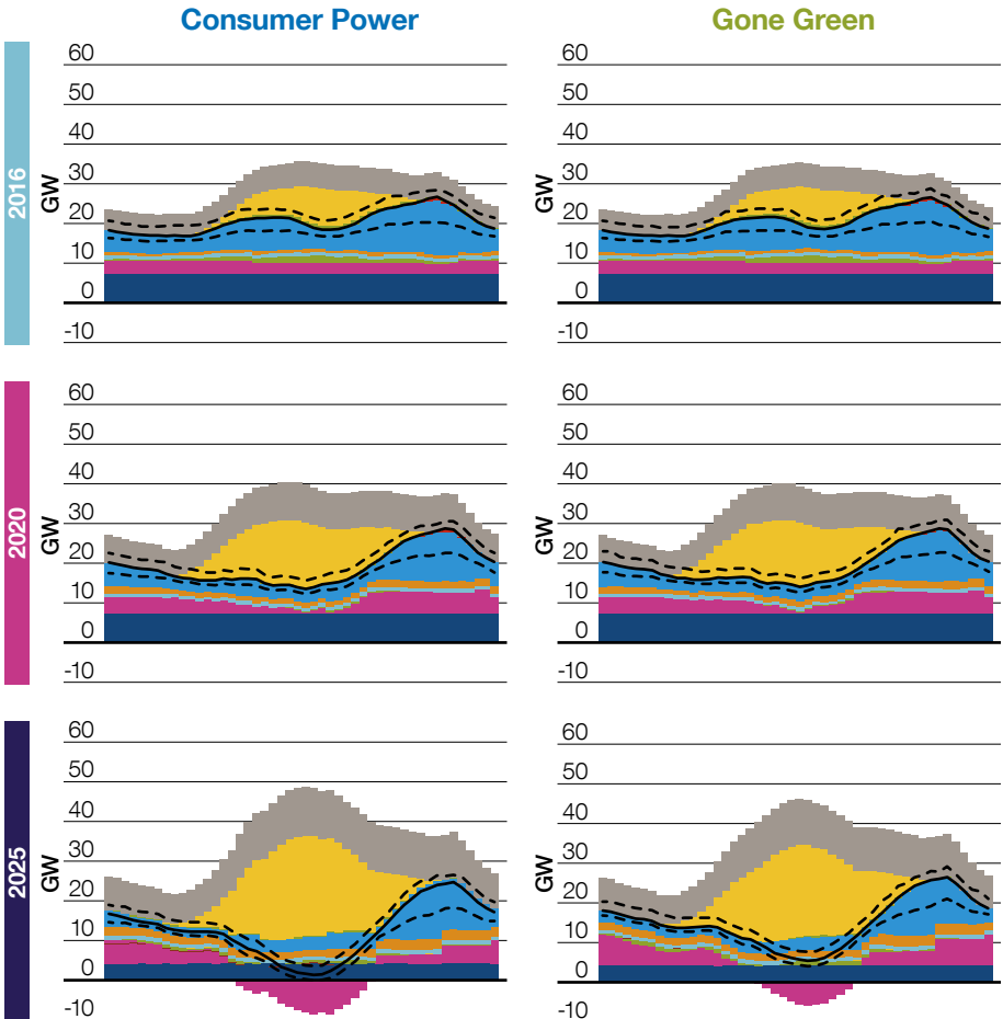
Figure 2.10 Generation dispatch, summer minimum demand
