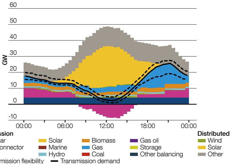
Figure 2.9 Generation dispatch example, summer, Consumer Power
