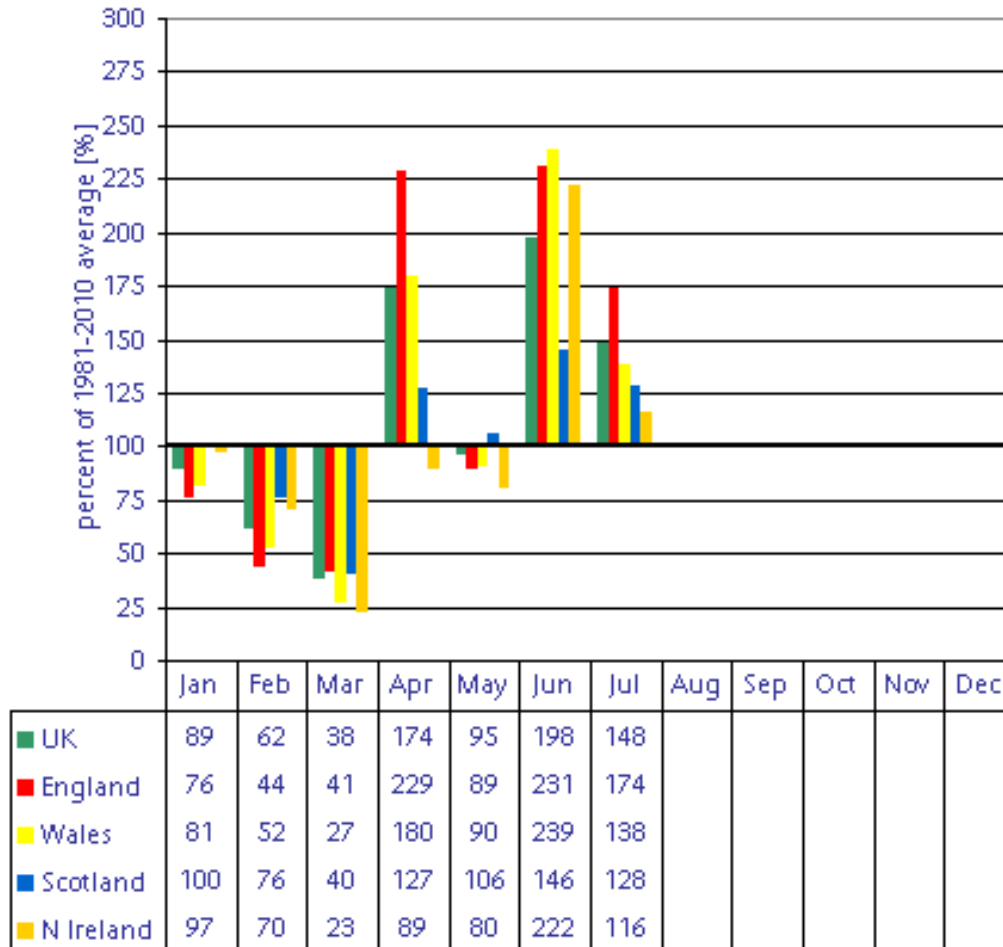
Rainfall (1981-2010) anomalies for 2012
