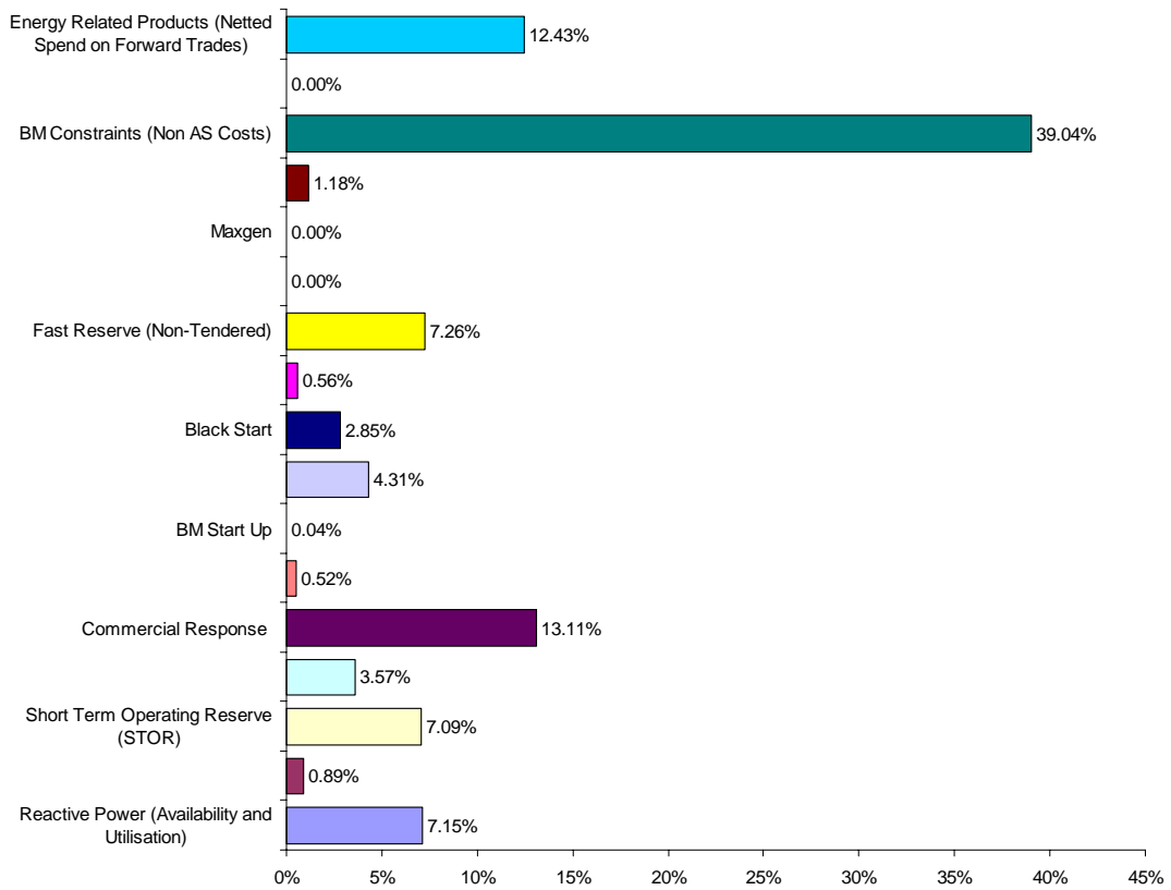
Summary of Balancing Services Costs March 2015
