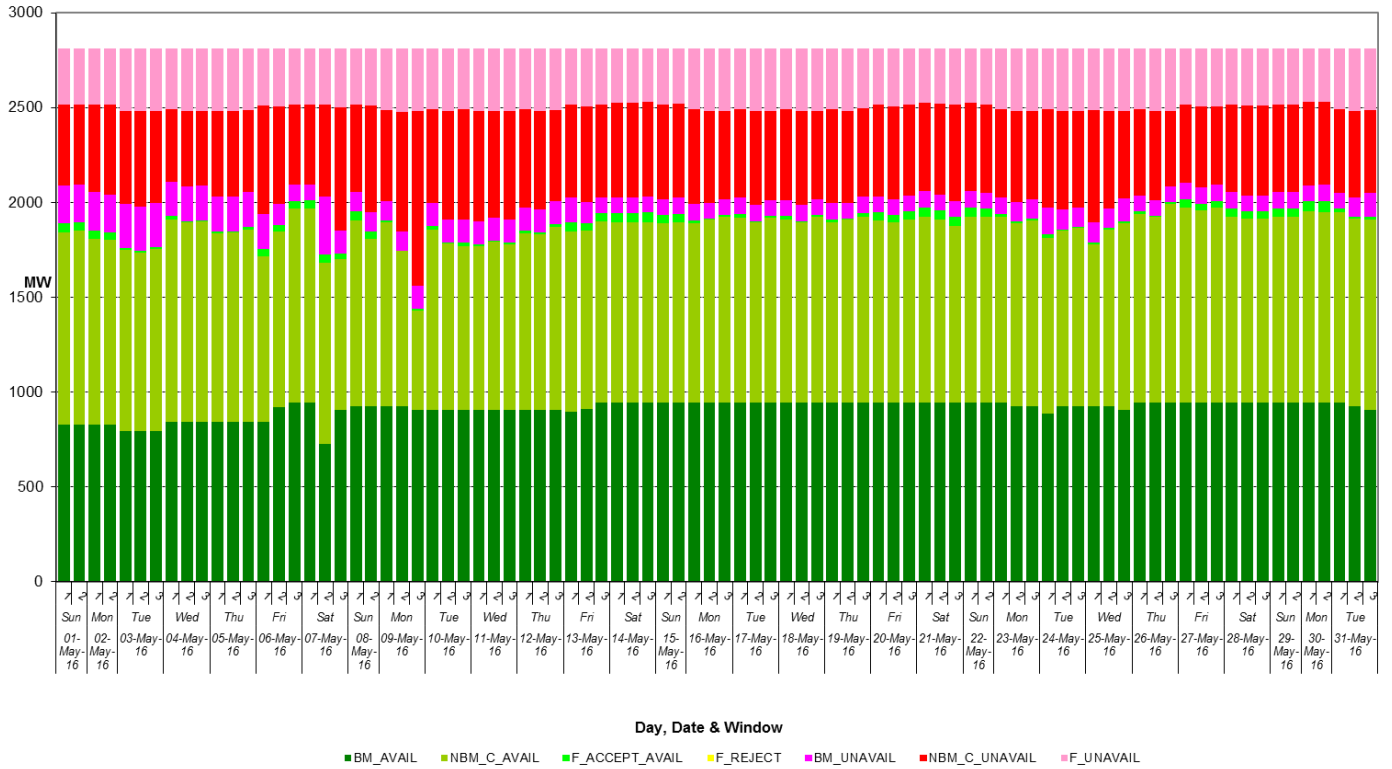
STOR MW Profile for month of May 2016
