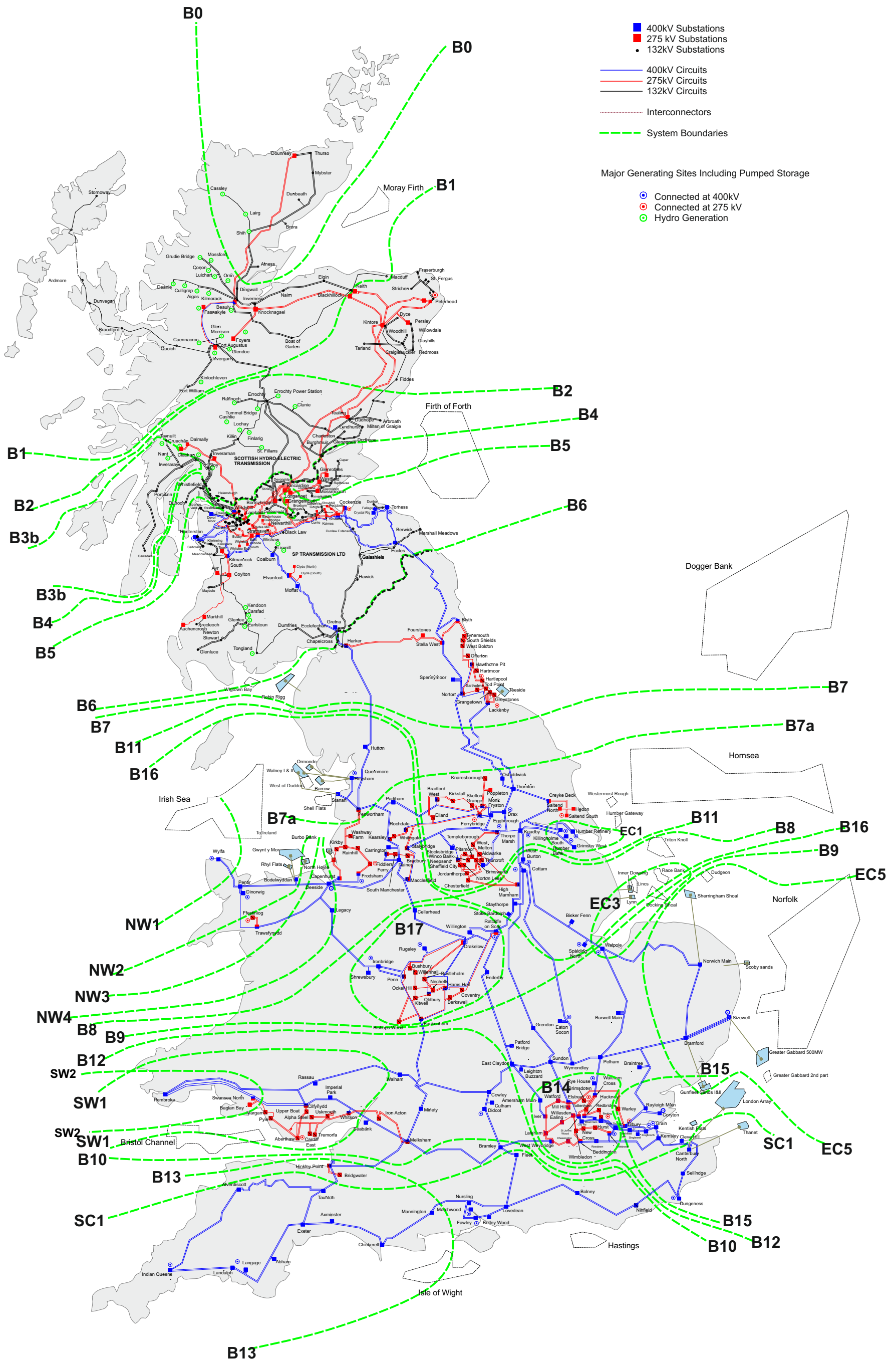
Figure A1.2: GB Transmission System Boundaries
