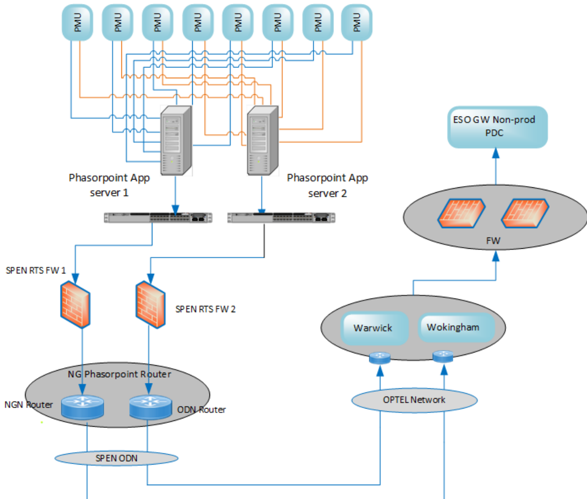
Figure 1 Architecture, for PMU data transfer to the NESO PDC through SPEN Transmission Owner PDC
