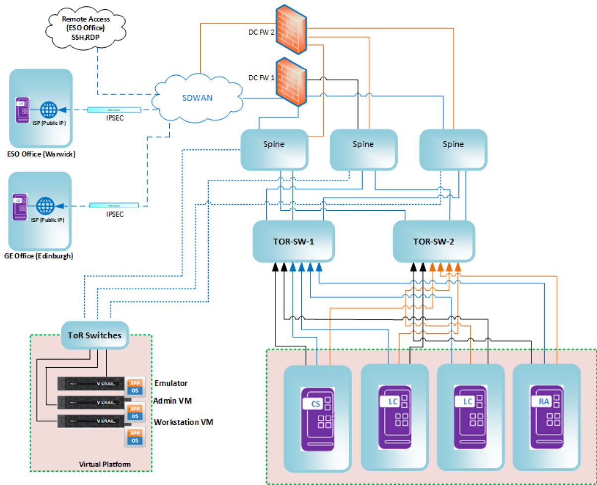
Figure 2 MCS system arrangement installed in a Data Centre.
