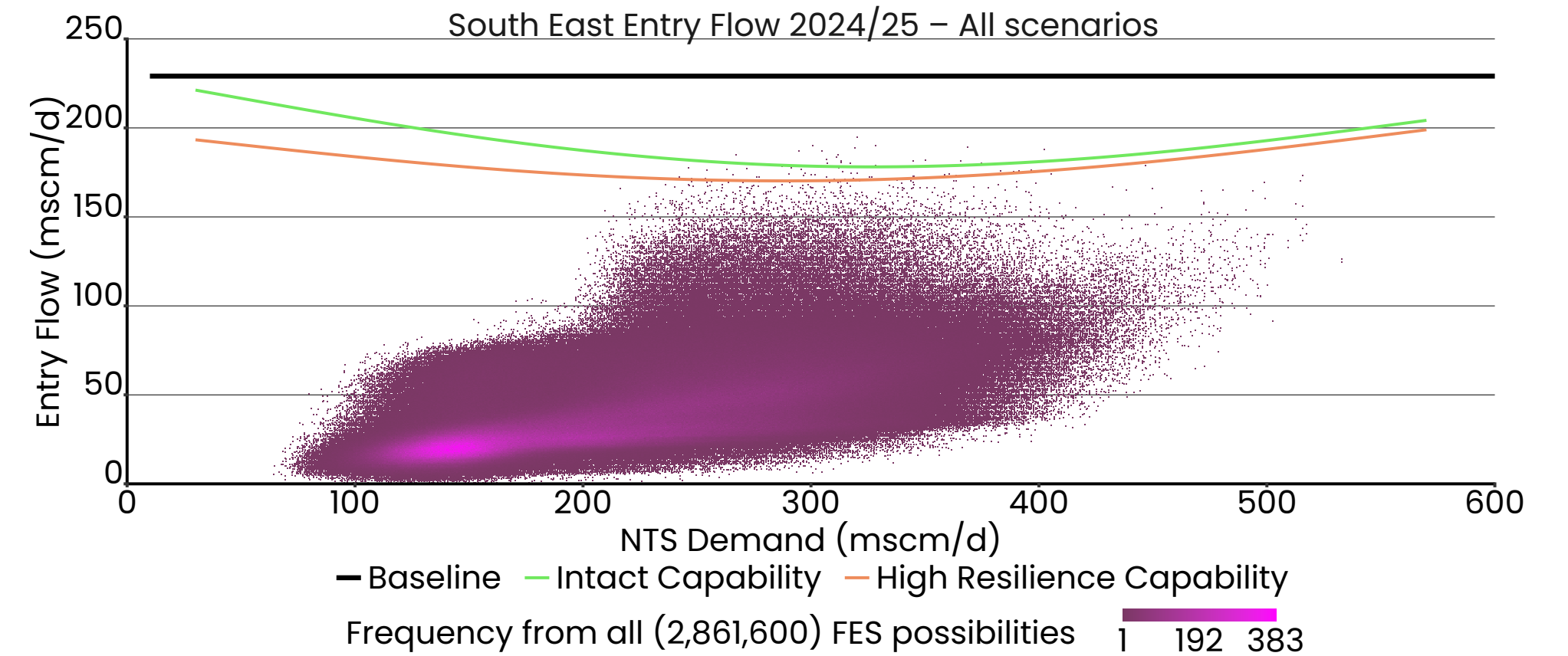
Figure 27: South East (Zone 7) Optimisation entry flame charts
