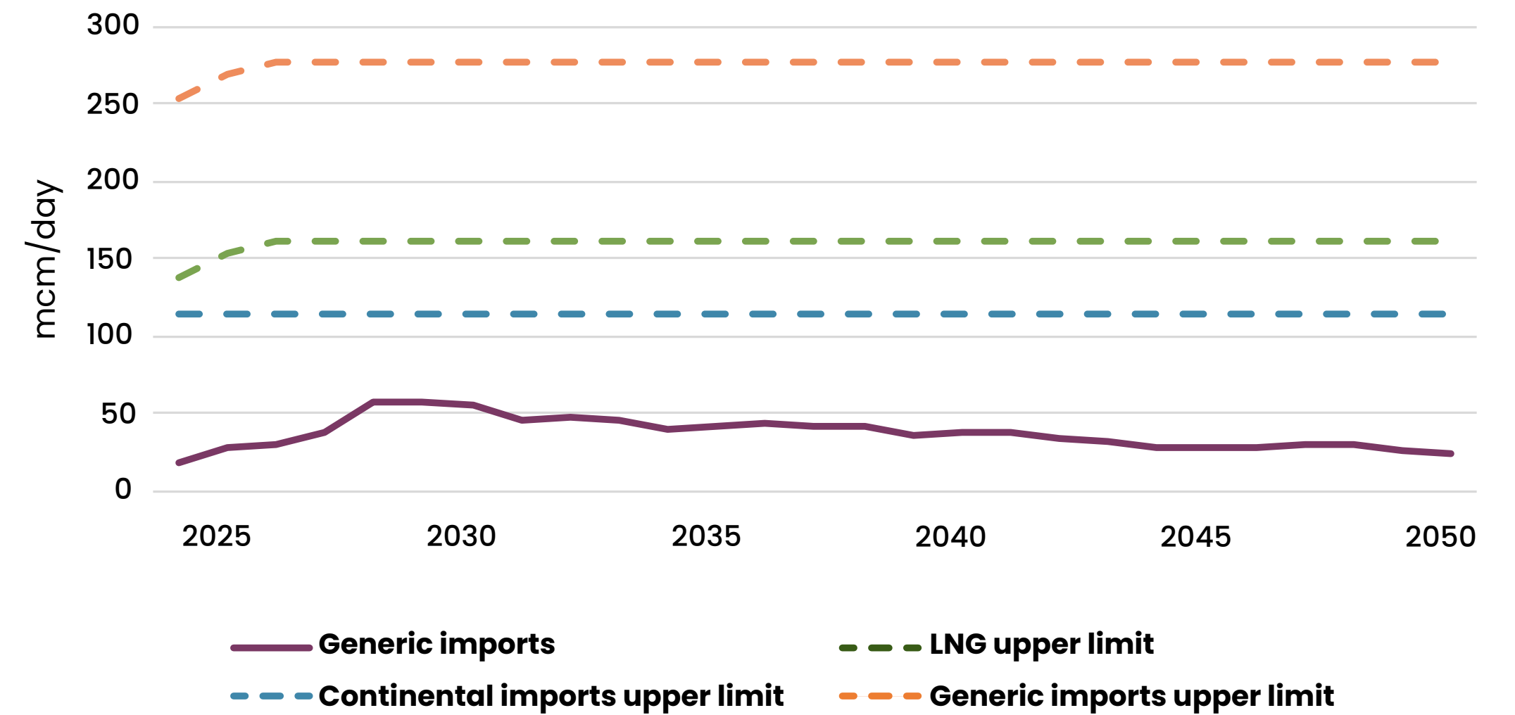
Figure 32: FES 2024 gas supply ranges (Generic imports supply)
