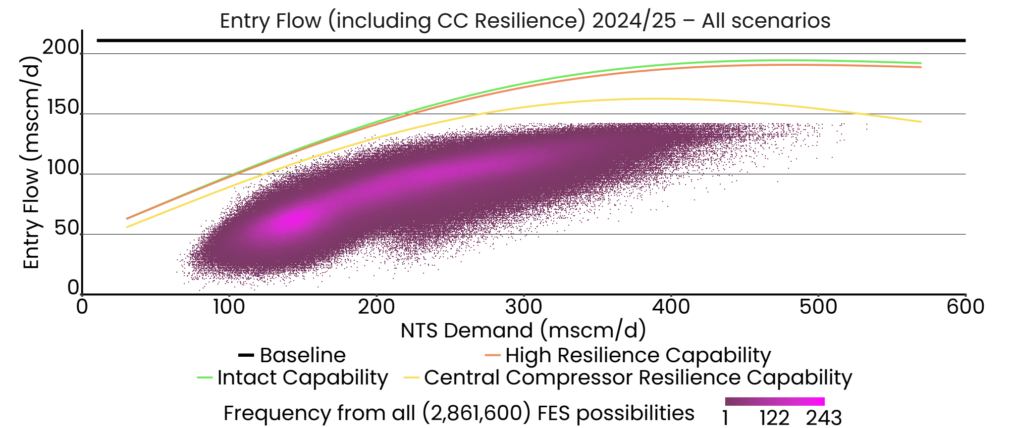
Figure 9: Flame charts for RIIO Zone 1 entry with CC resilience
