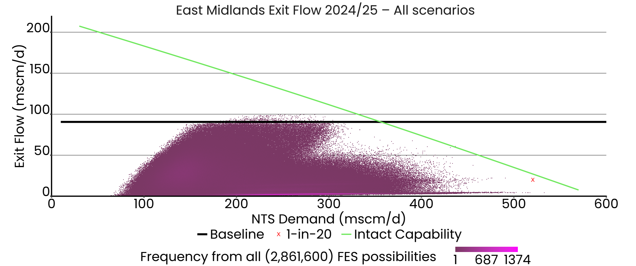
Figure 21: Sensitivity 1: RIIO Zone 6 exit (overall) flame charts
