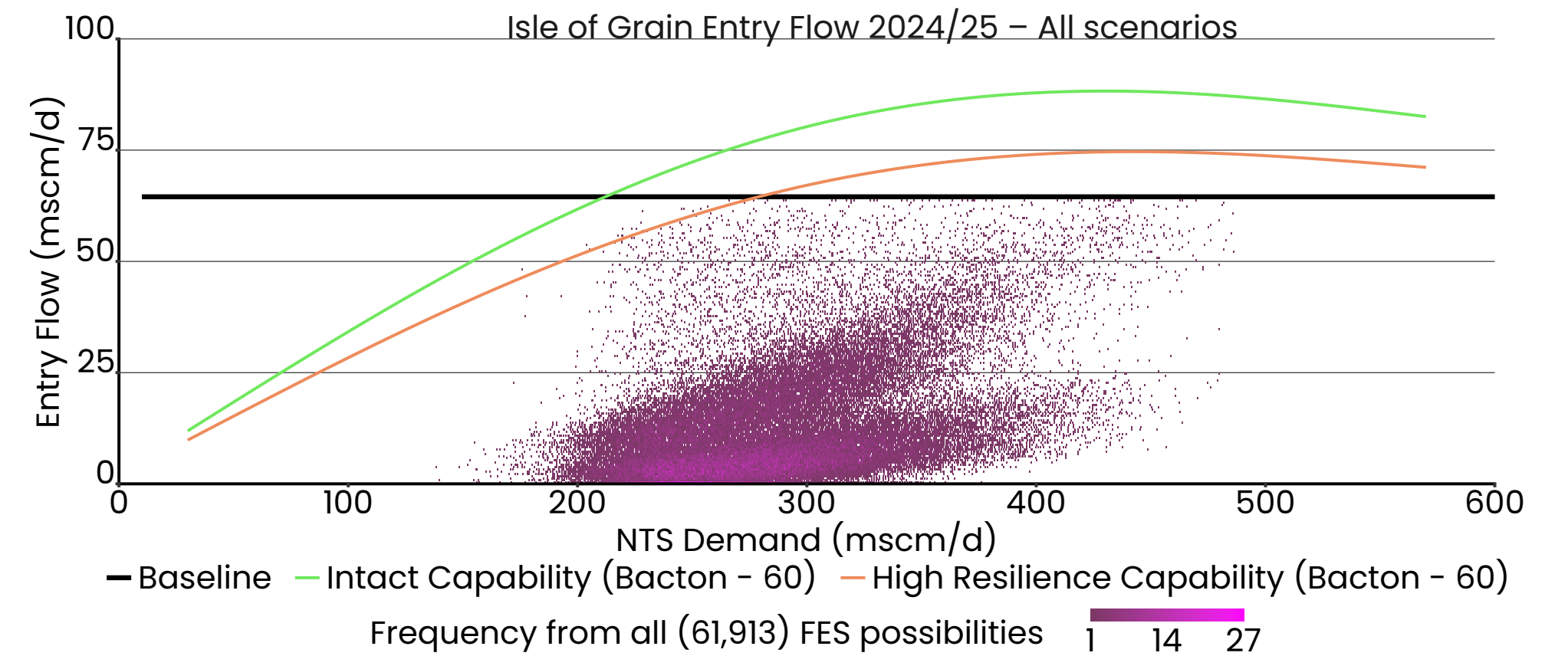
Figure 26: South East (Zone 7) Isle of Grain entry flame charts
