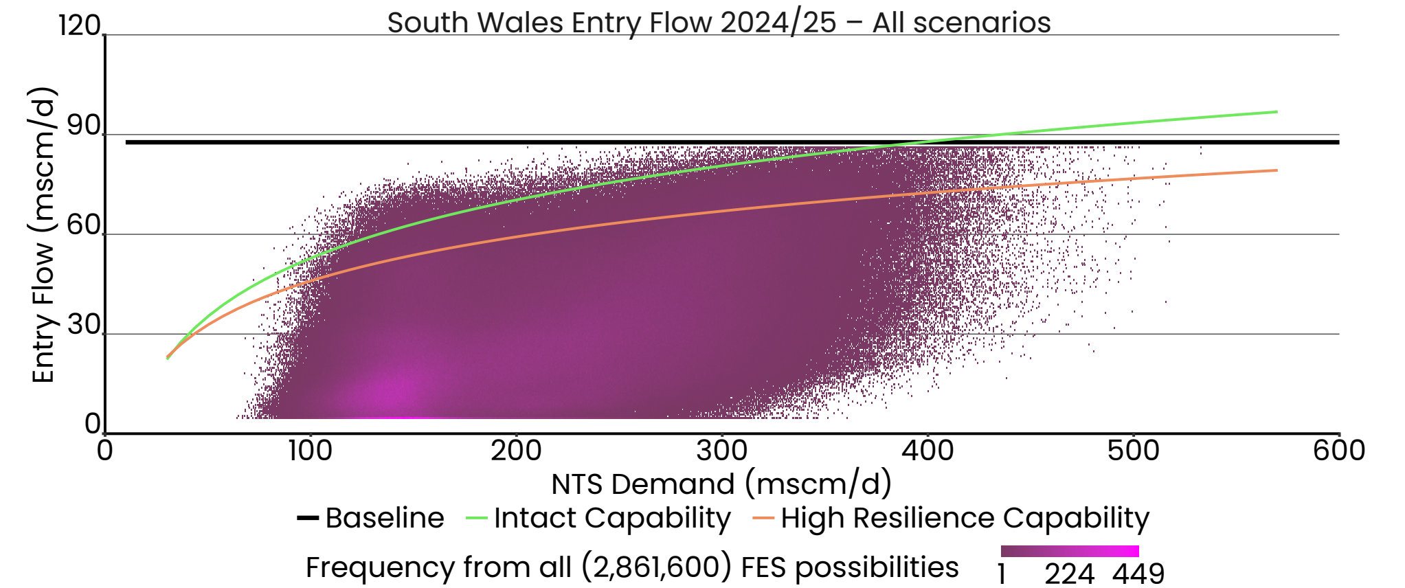
Figure 16: South Wales (Zone 4) entry flame charts
