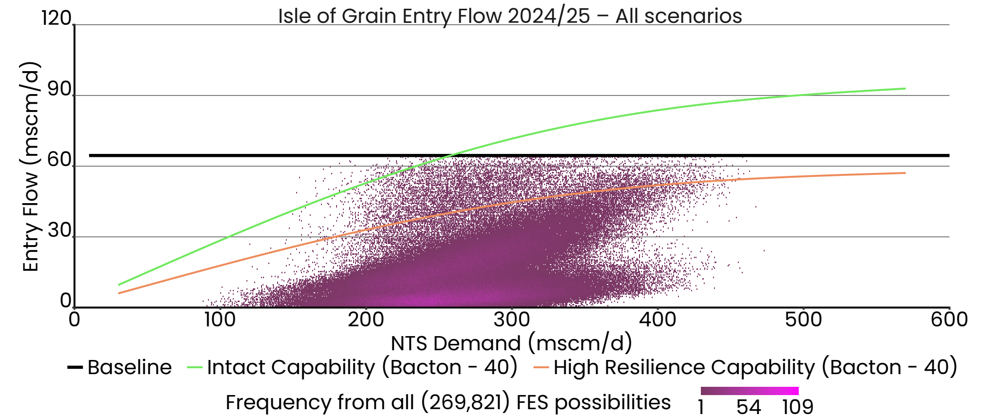
Figure 25: South East (Zone 7) Isle of Grain entry flame charts
