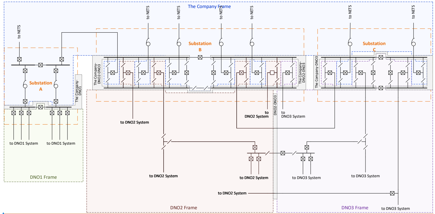
Figure 1010 - The Frames and Boundaries of the small system example
