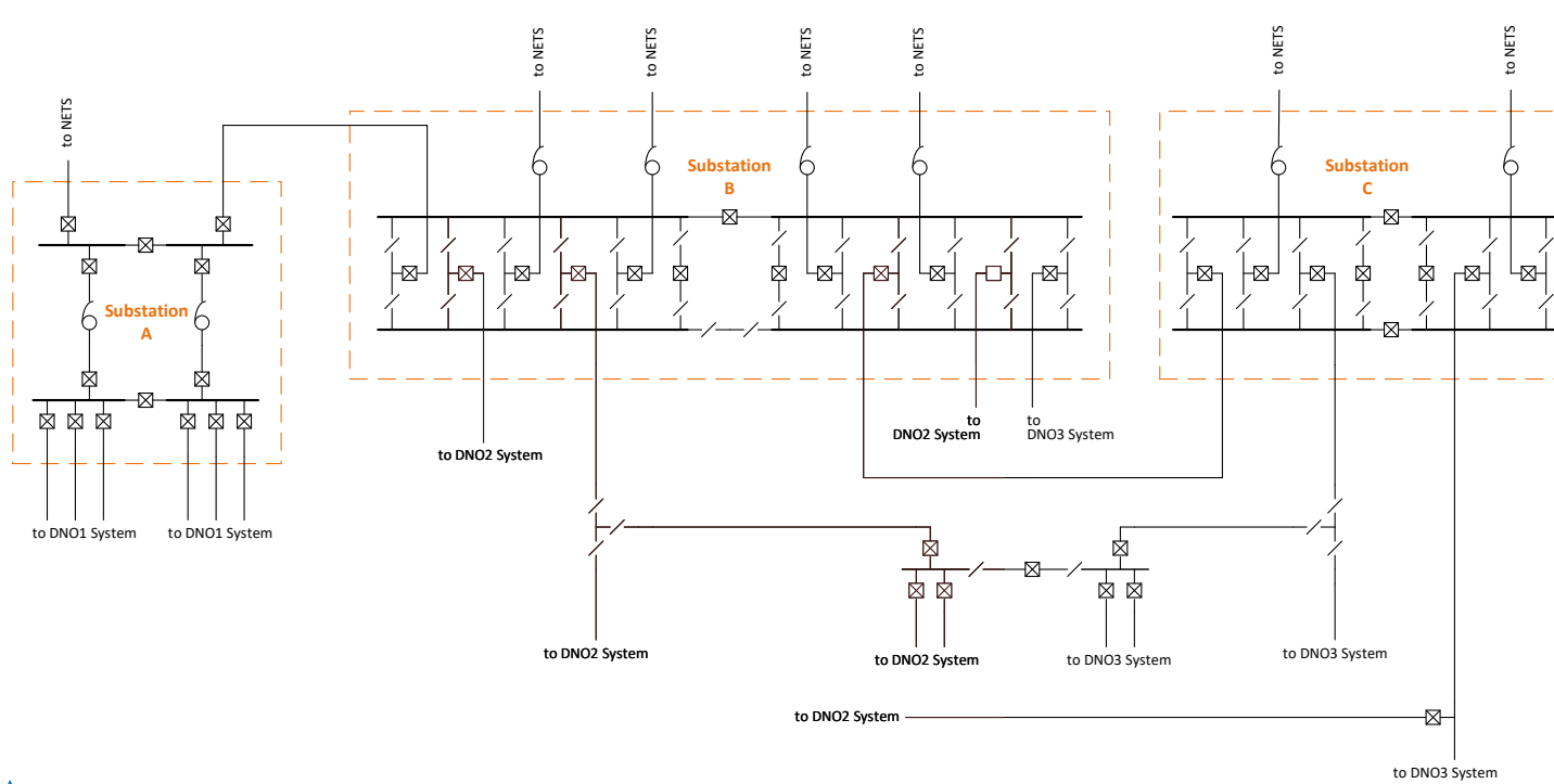
Figure 777 - Schematic of the small system example
