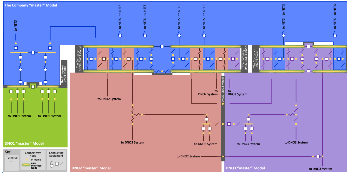
Figure 11114 – Major grid objects comprising the master Structural Models which 'fit into' each Frame and Boundary
