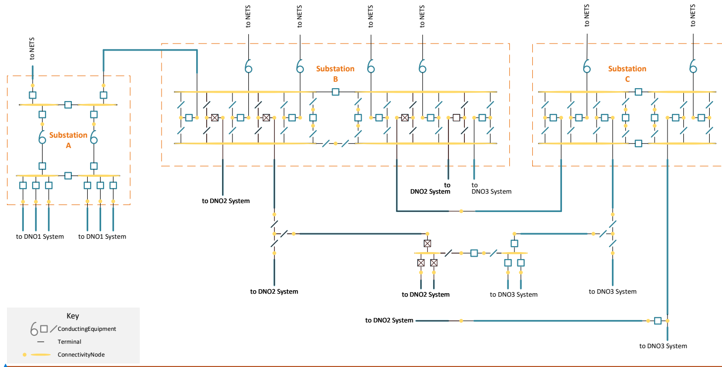
Figure 88 – Foundational grid objects used to represent the equipment and connectivity of small system example
