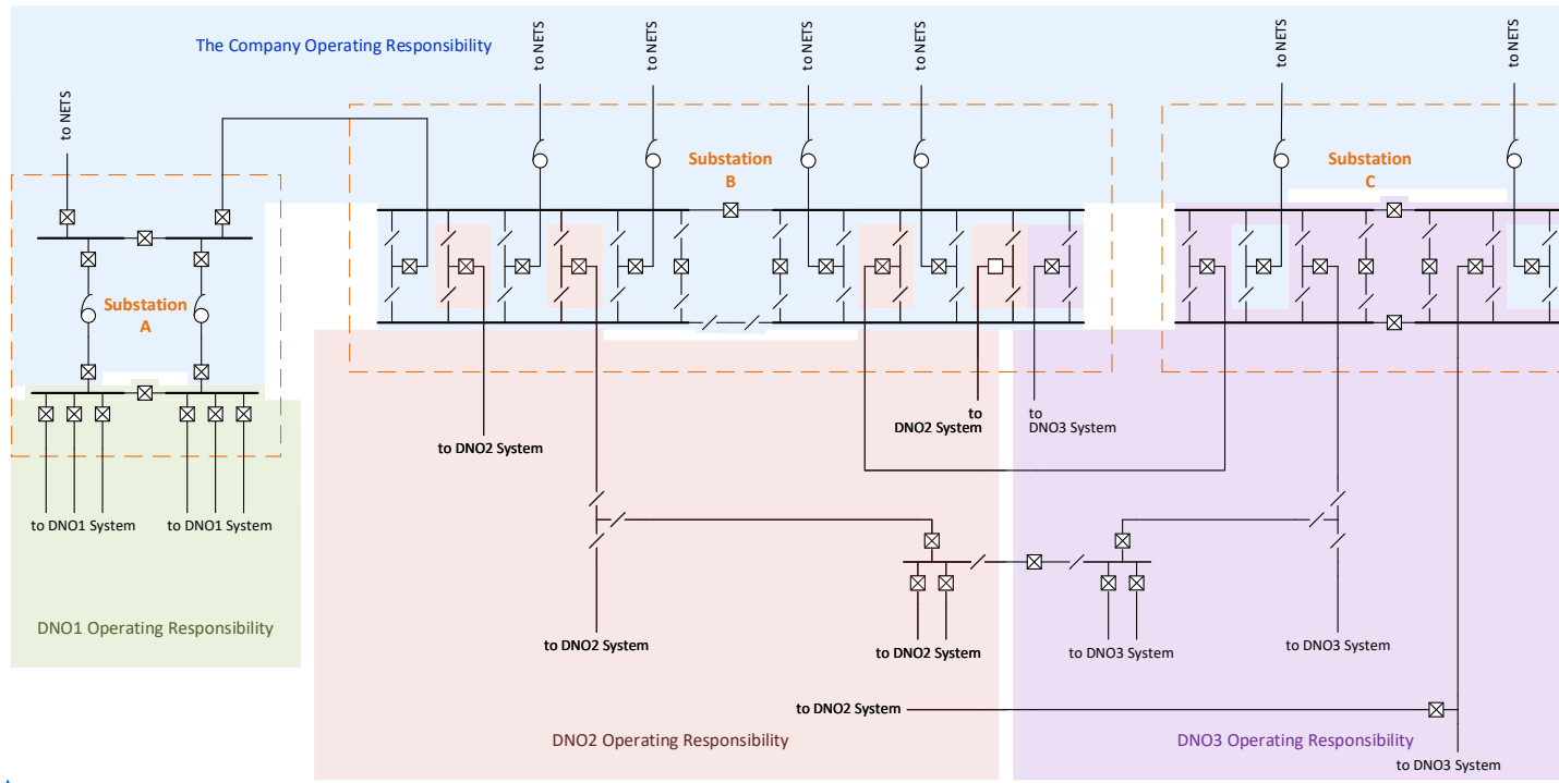
Figure 999 – Allocation of operating responsibility for the small system example
