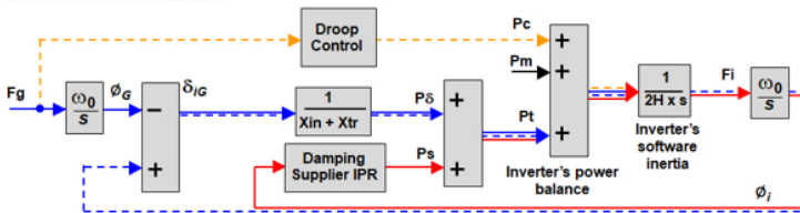
Figure PC.A.5.8.1 (b) – Preferred simplified diagram of a system with a droop control ability that can add Control-Based Active Droop Power . This diagram does not add extra closed loop damping to the GBGF-I's closed loop function shown by the solid red line and the dotted blue line.
