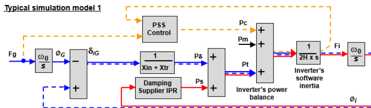
Figure PC.G.4.1.1 (a) Preferred simplified diagram of a GBGF-I with a Power System Stabiliser "PSS" that can add damping to the GBGF-I's closed loop function shown by the solid red line and the dotted blue line.
