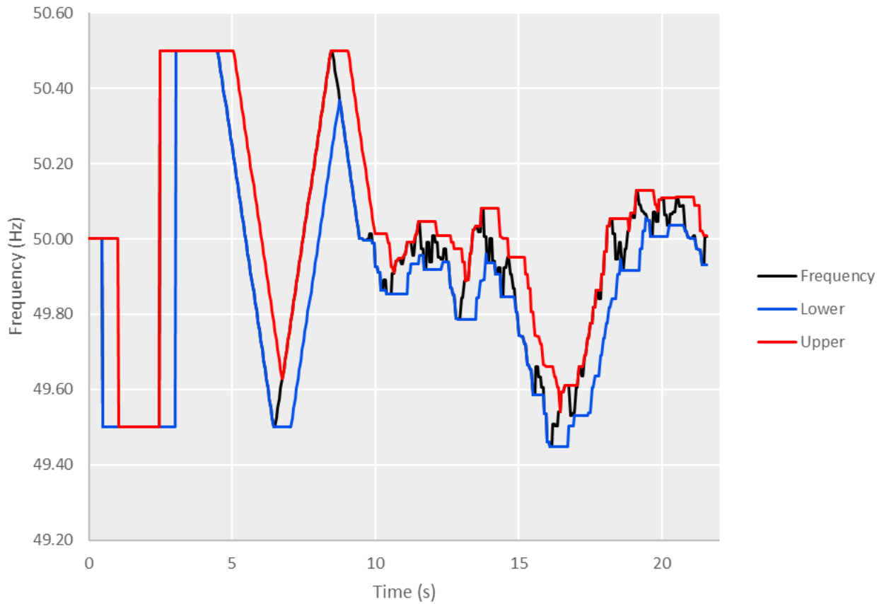
Figure 3: Example of frequency bounds calculation
