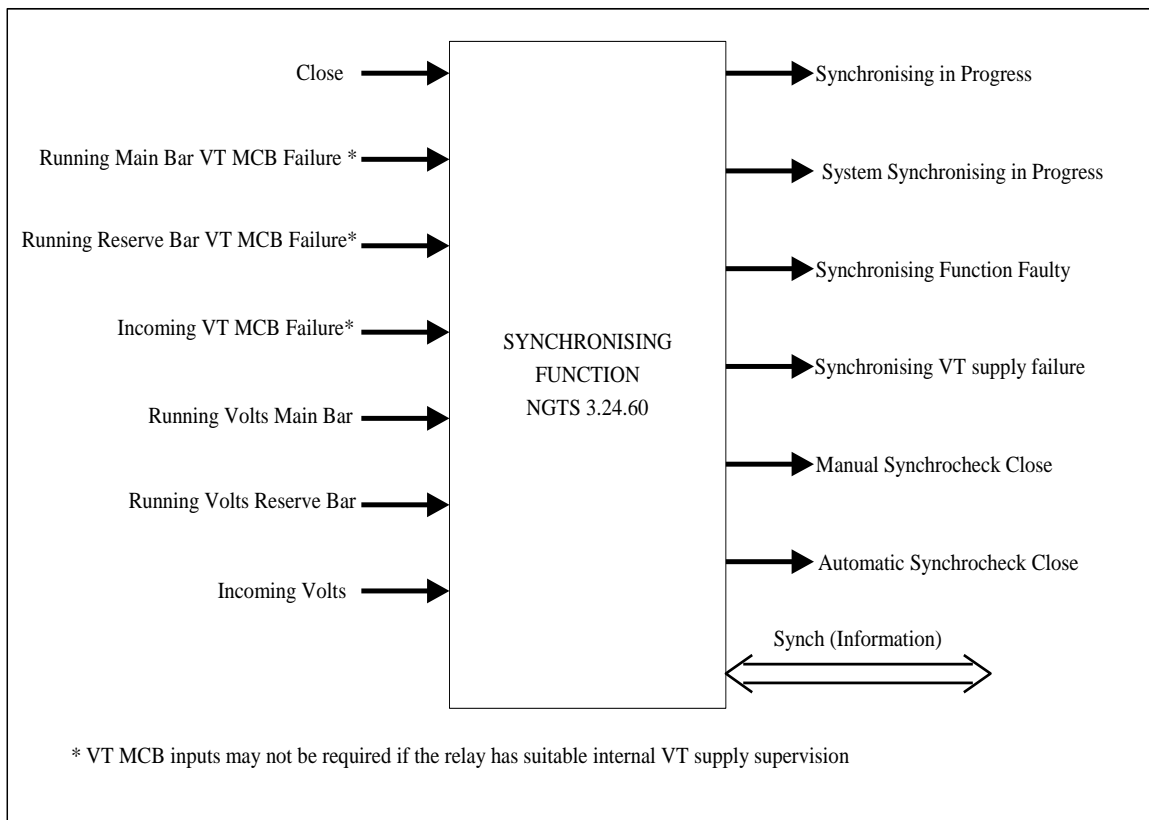
Figure 1: Synchronising Functional Interfaces
