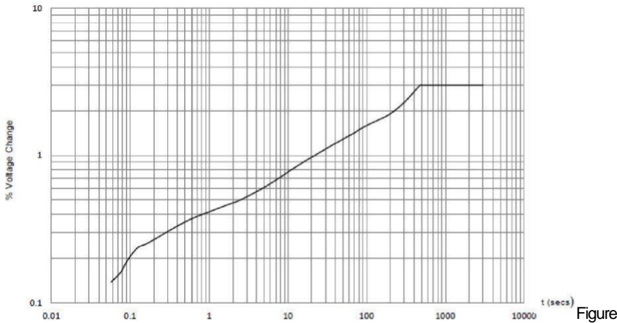
6.1 Maximum Voltage Step Changes Permitted for Operational Switching derived from ER P28 B.1.2
