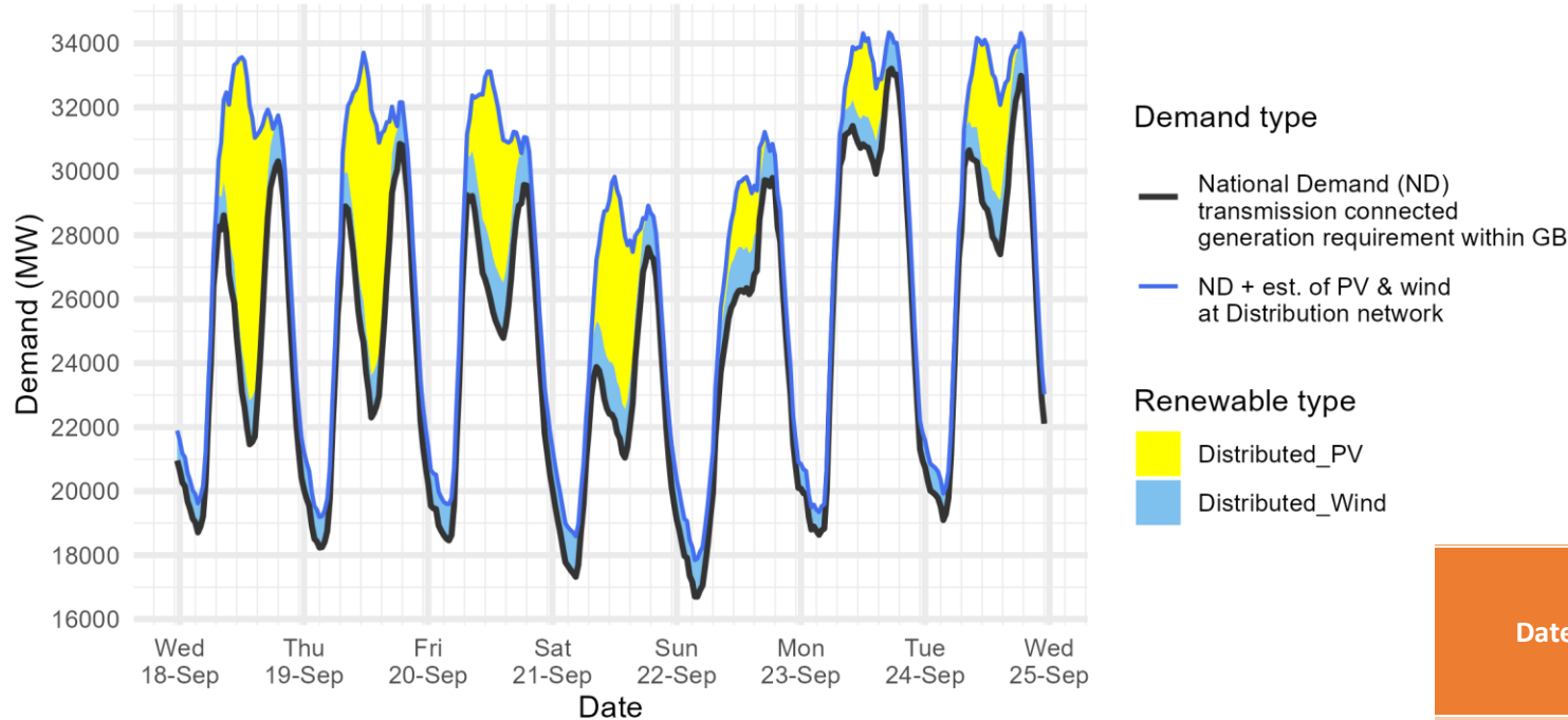
ESO National Demand outturn 18-24 September 2024
