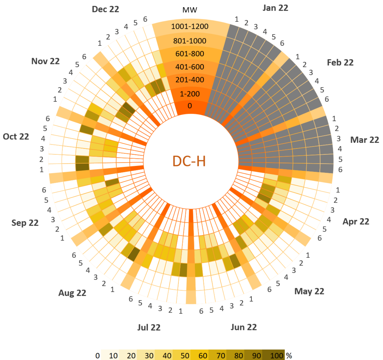
Figure 4: Indicative DC-H Requirements 2022
