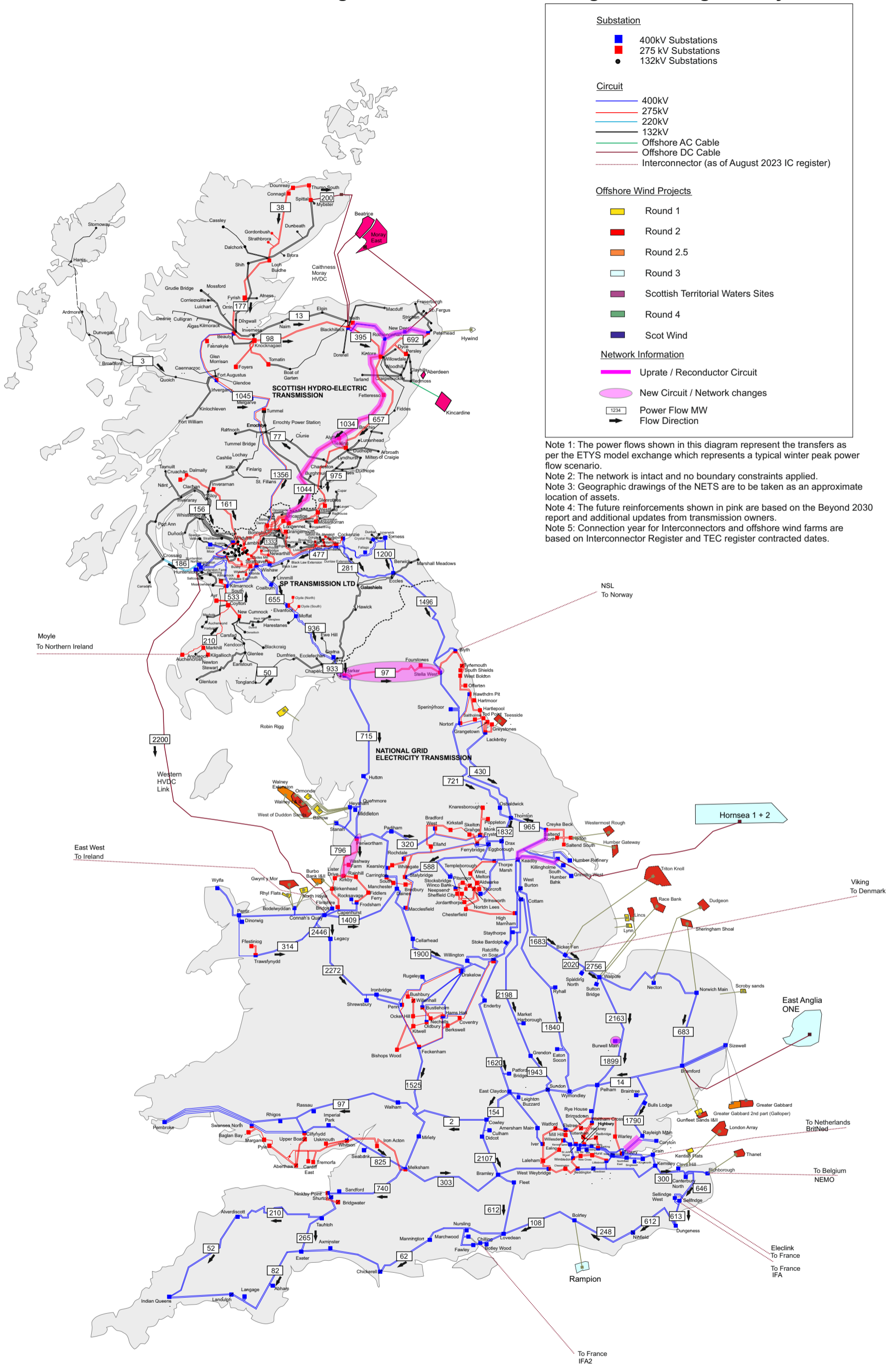
Figure C1: GB Power Flow Diagram Leading the Way 2023/24
