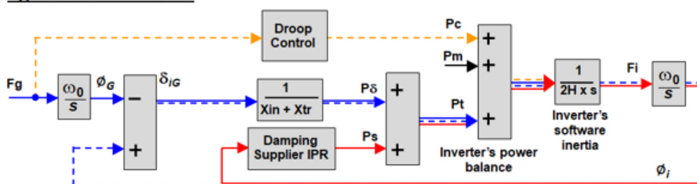
Figure PC.A.5.8.1 (a) Preferred simplified diagram of a GBGF-I with a Power System Stabiliser "PSS" that can add damping to the GBGF-I's closed loop function shown by the solid red line and the dotted blue line.
