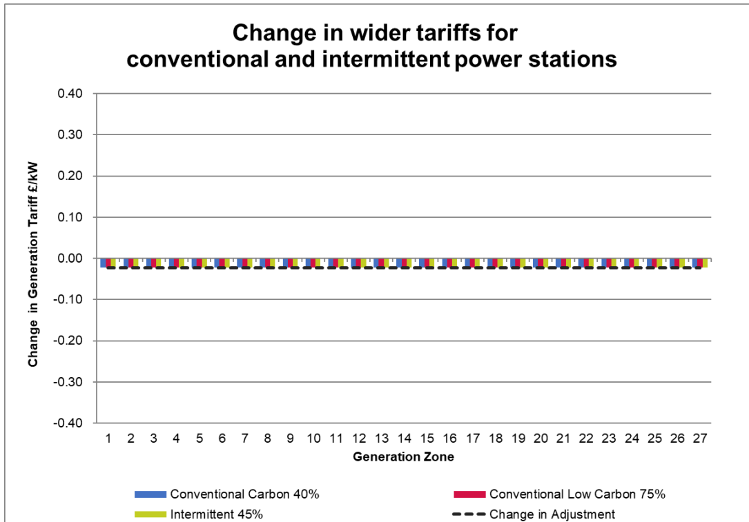
Figure 1 Variation in generation wider zonal tariffs
