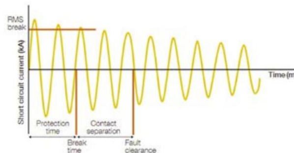
Figure D2.1 – AC component of the short-circuit current.
