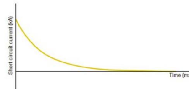
Figure D2.2 – DC component of the short-circuit current
