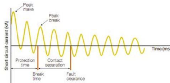
Figure D2.3 – Combined AC and DC components of the short-circuit current
