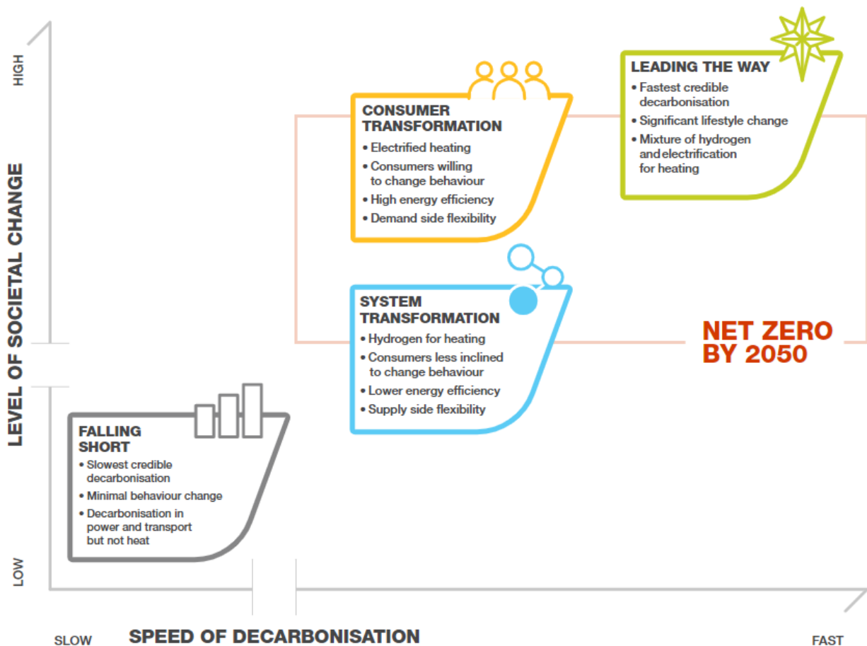
Figure 2: FES 2022 Scenarios
