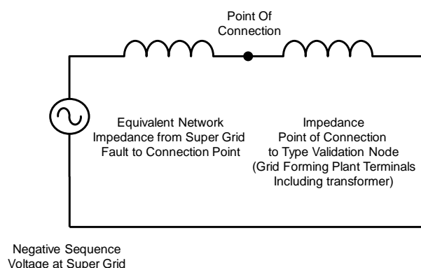
Figure I-2 – Simplified network diagram for NPS
