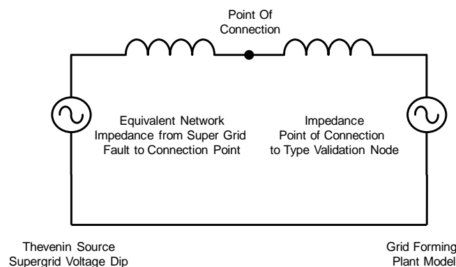
Figure I-1 – Simplified network diagram for PPS
