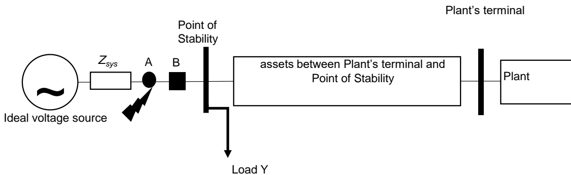
Figure 7: Network representation for Active RoCoF Response Power and Active Phase Jump Power extreme condition
