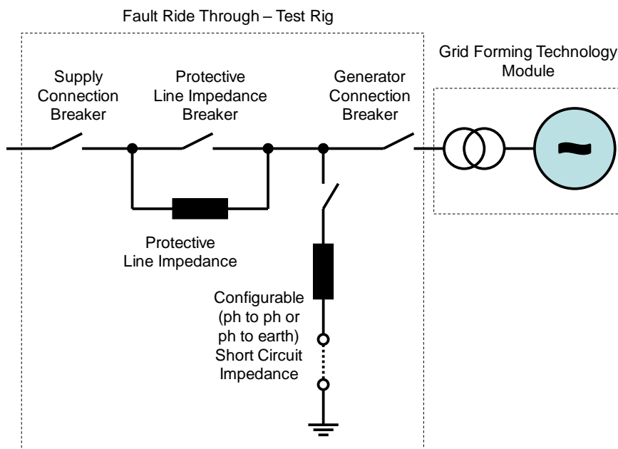
Figure G-2 – Fault ride through test rig single line diagram
