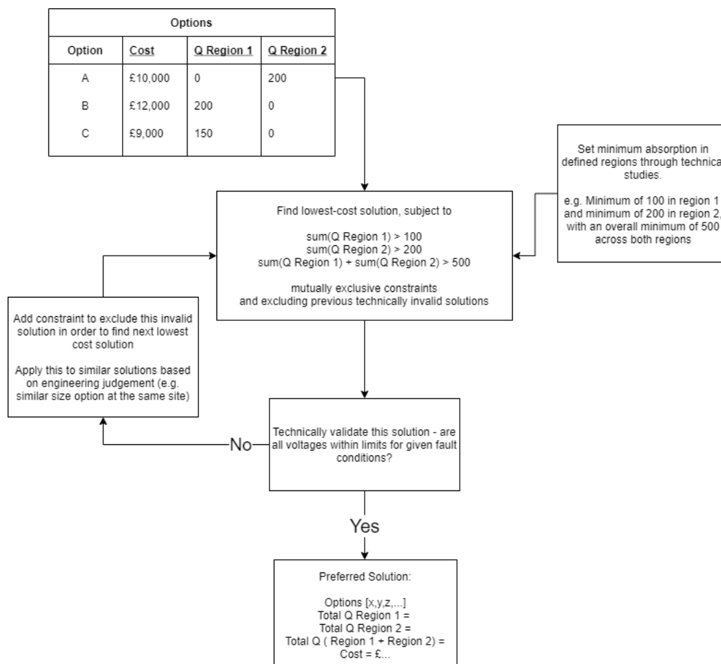
Figure 6.14: Example Joint technical and economic optimisation process
