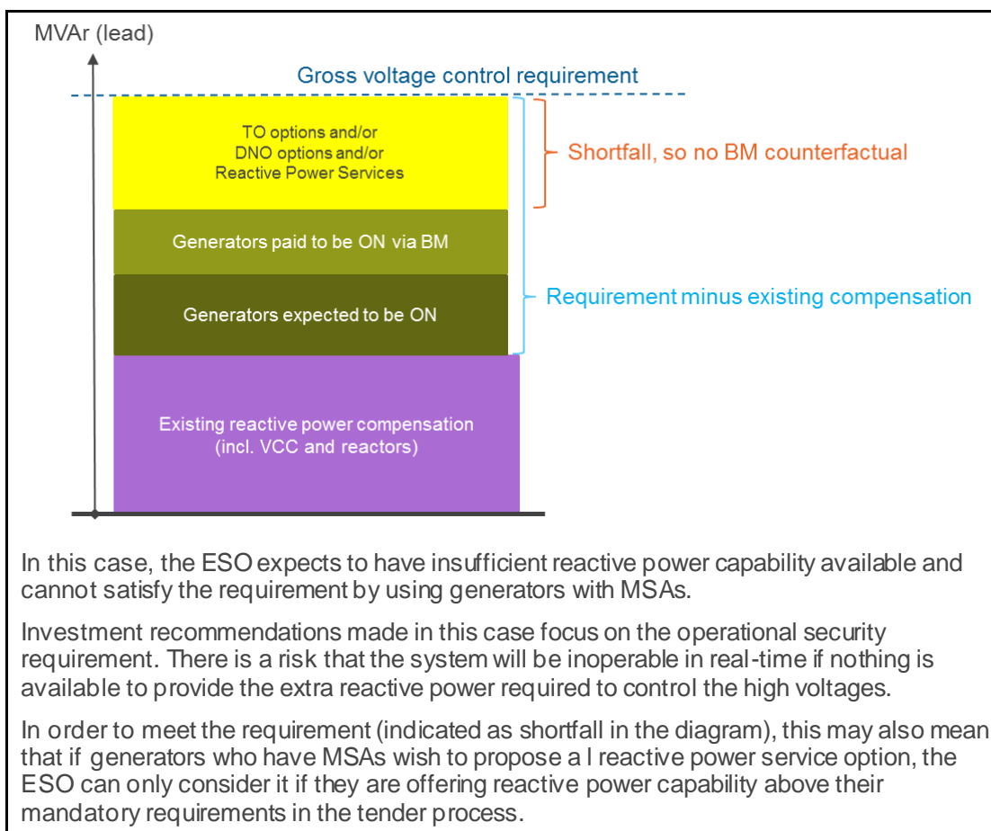
Figure 6.3 Proposed options providing the reactive power needed to meet voltage control requirement as sufficient services cannot be procured from the BM
