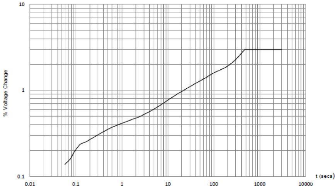
6.1 Maximum Voltage Step Changes Permitted for Operational Switching
