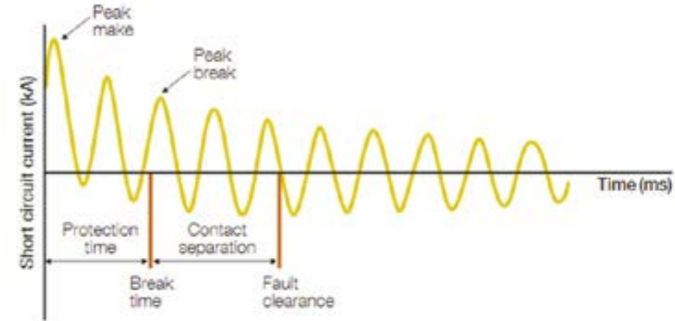
Figure D2.3 Combined AC and DC components of short-circuit current
