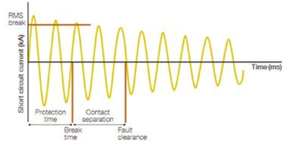
Figure D2.1 AC component of the short-circuit current
