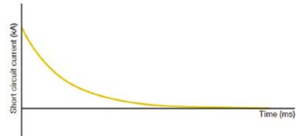
Figure D2.2 DC component of the short-circuit current
