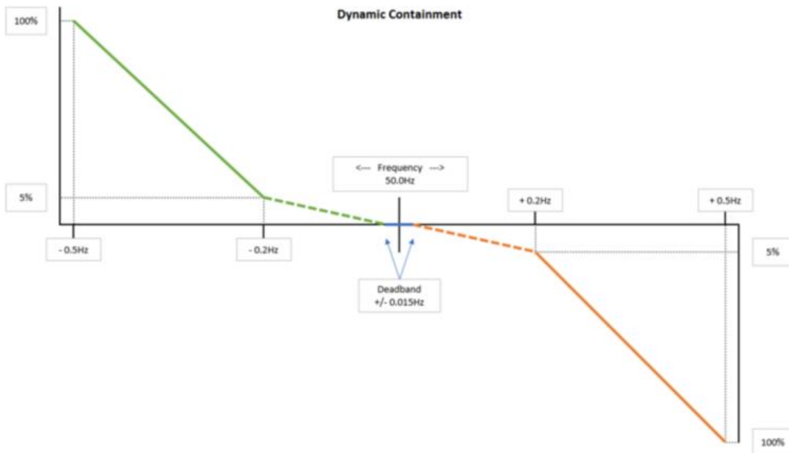
Figure 1 – Dynamic Containment Delivery Requirements
