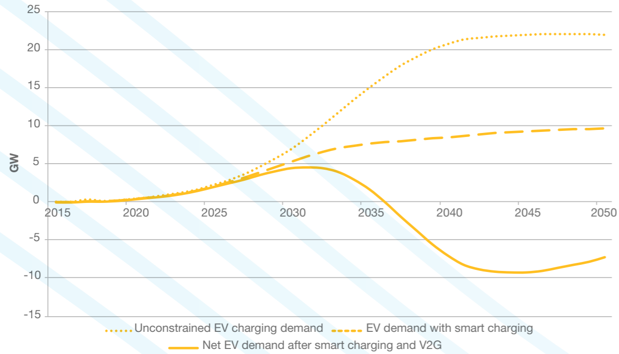
Figure SV.42: Electric vehicle charging behaviour at ACS 2 winter peak system demand
