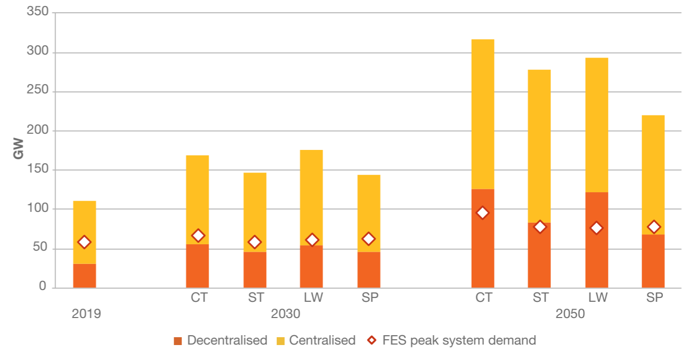
Figure SV.25: Connection location of installed generation capacities and peak demand (excluding vehicle-to-grid)
