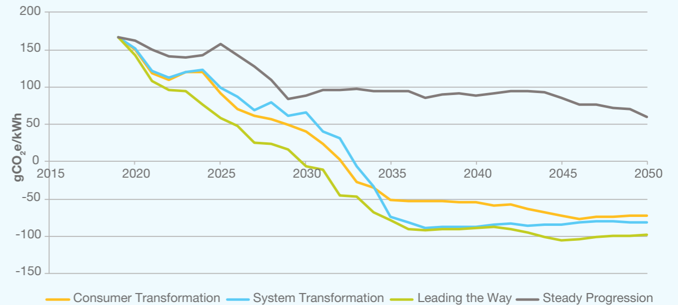
Figure SV.27: Power sector carbon intensity 2
