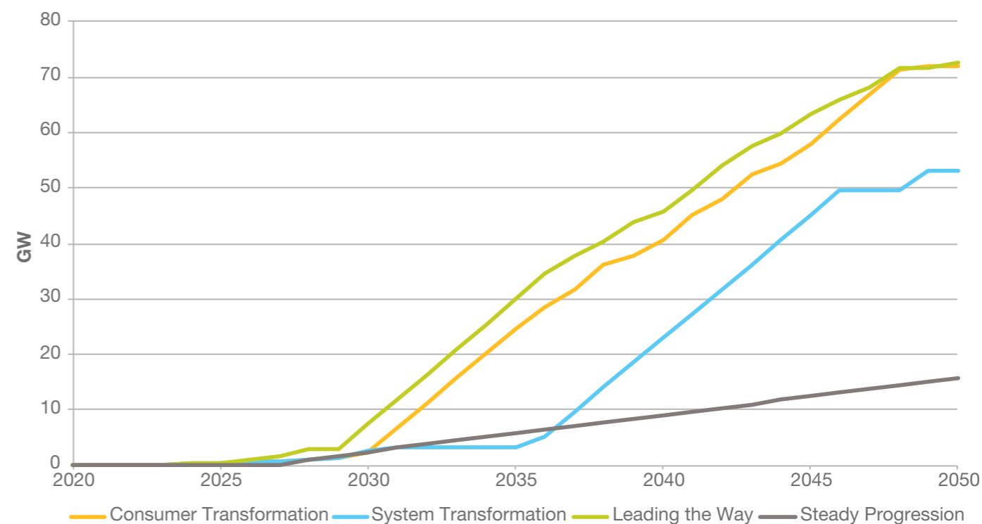
Figure SV.43: Installed onshore network-connected electrolysis capacity by scenario
