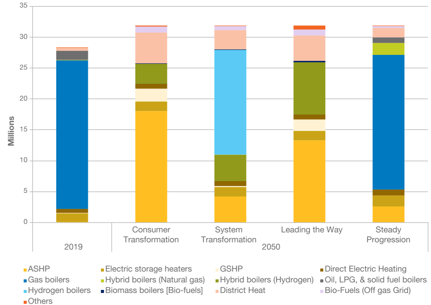
Figure CV.10: Overall home heating technology mix in 2050
