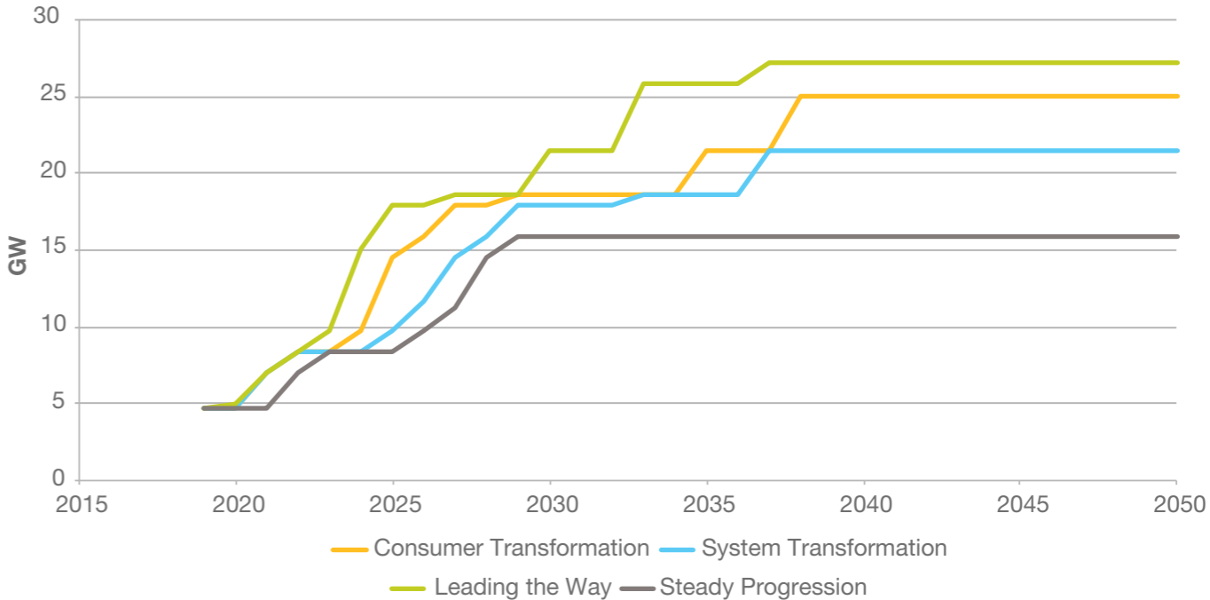
Figure SV.35: Installed interconnector capacity
