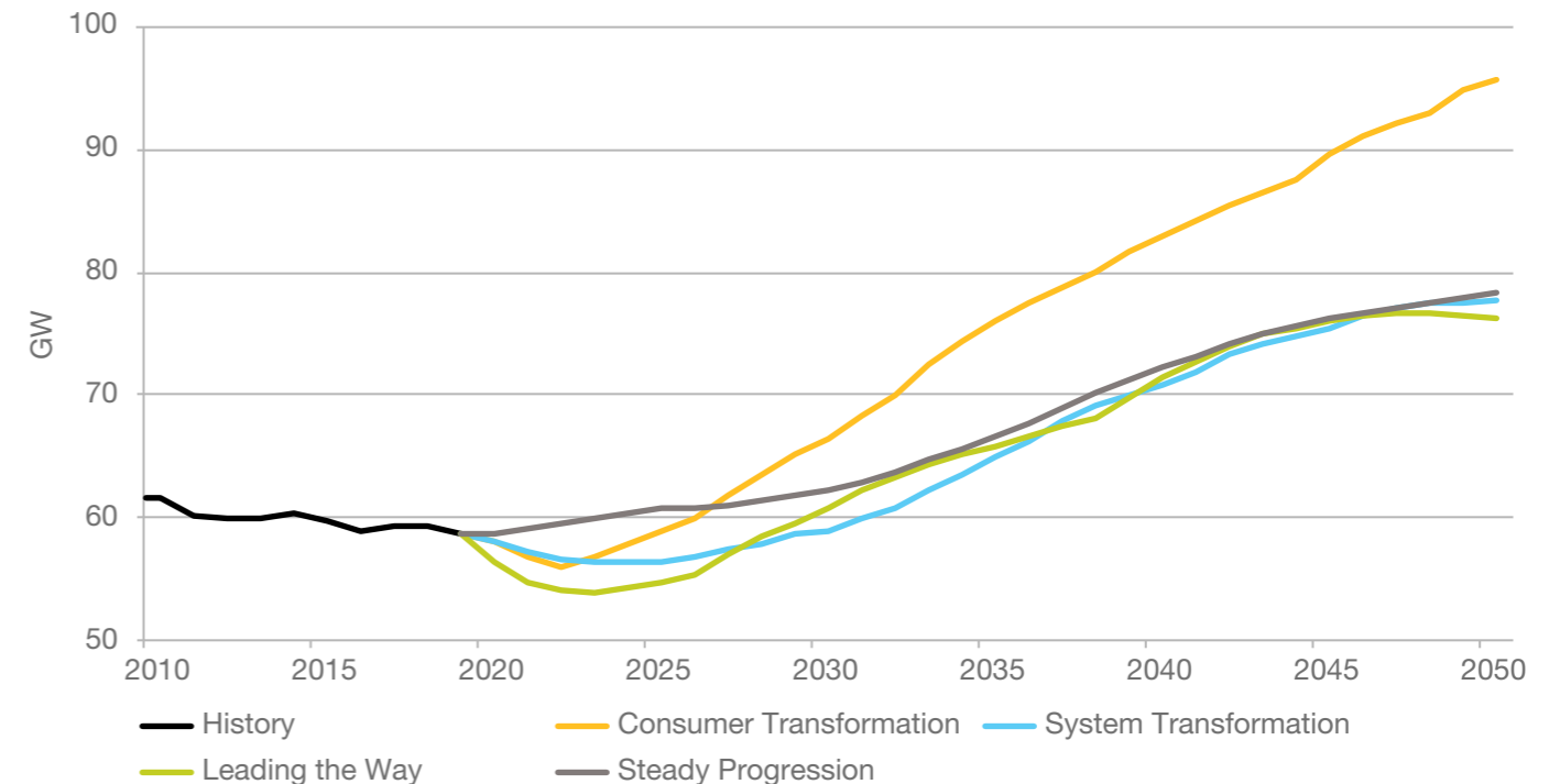
Figure SV.4: Electricity peak demand (including losses)
