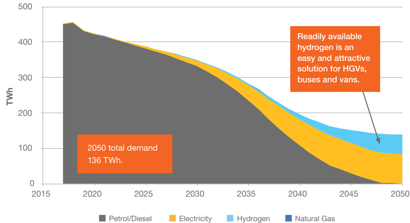
Figure CV.24: Annual energy demand for road transport in System Transformation
