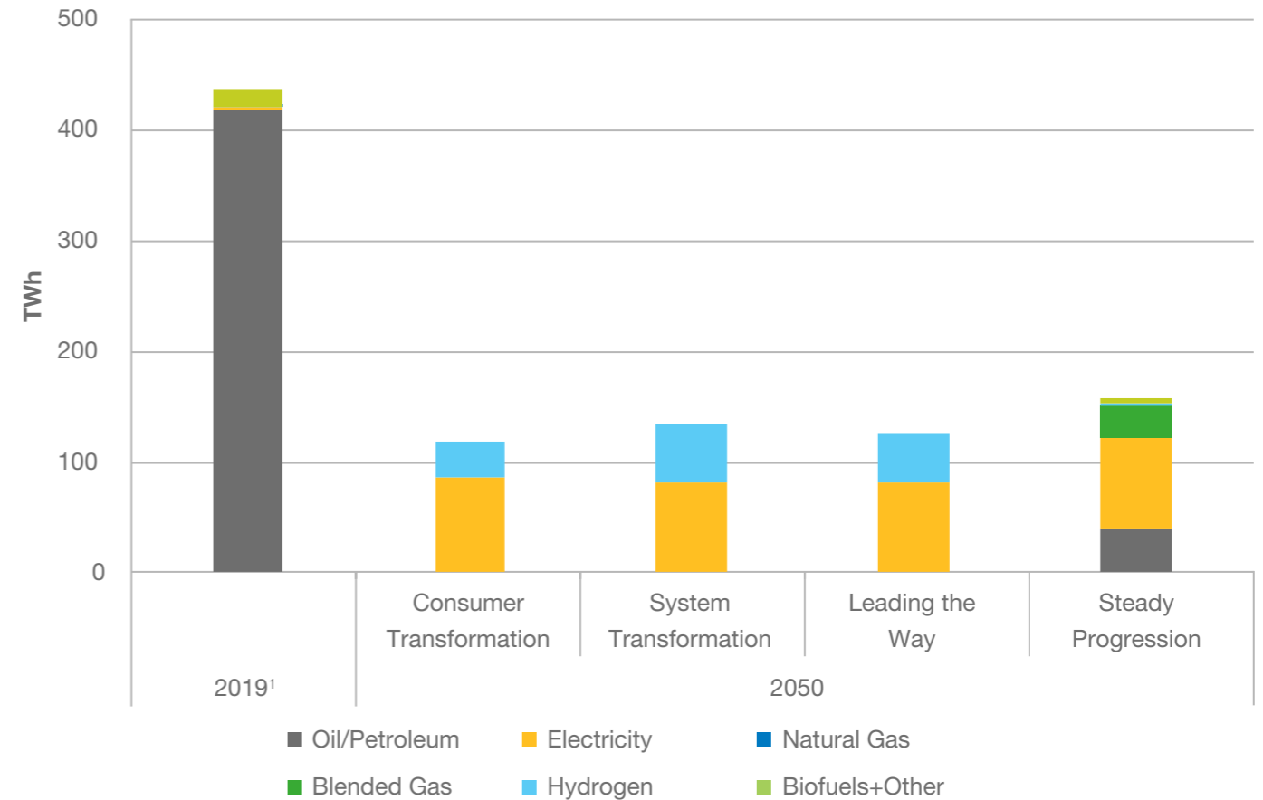
Figure CV.19: Total annual demand for road transport 1 in 2050
