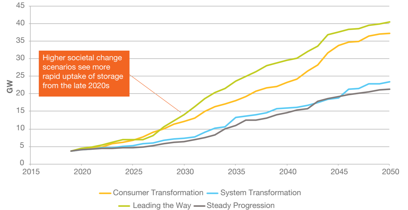
Figure SV.36: Installed electricity storage capacity 4
