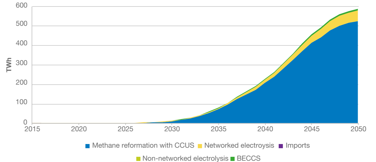
Figure SV.20: System Transformation hydrogen supply
