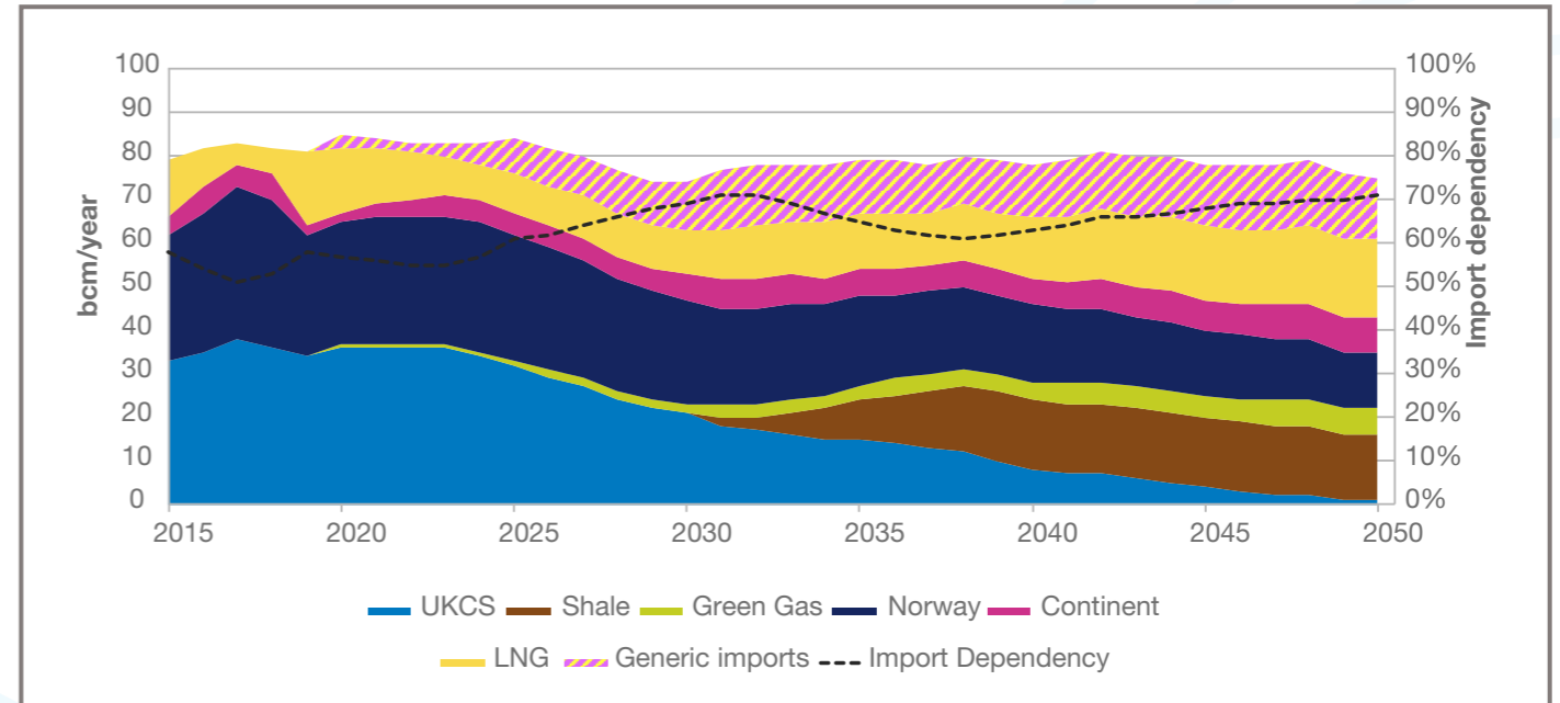
Figure SV.14: Annual gas supply in Steady Progression
