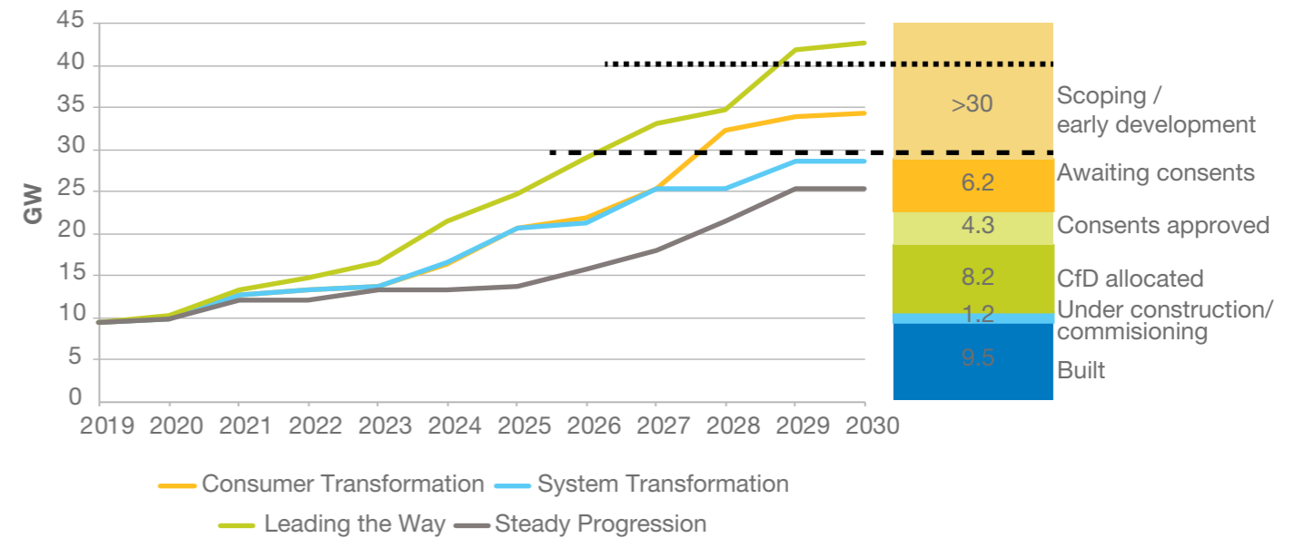
Figure SV.29: Potential offshore wind projects by scenario
