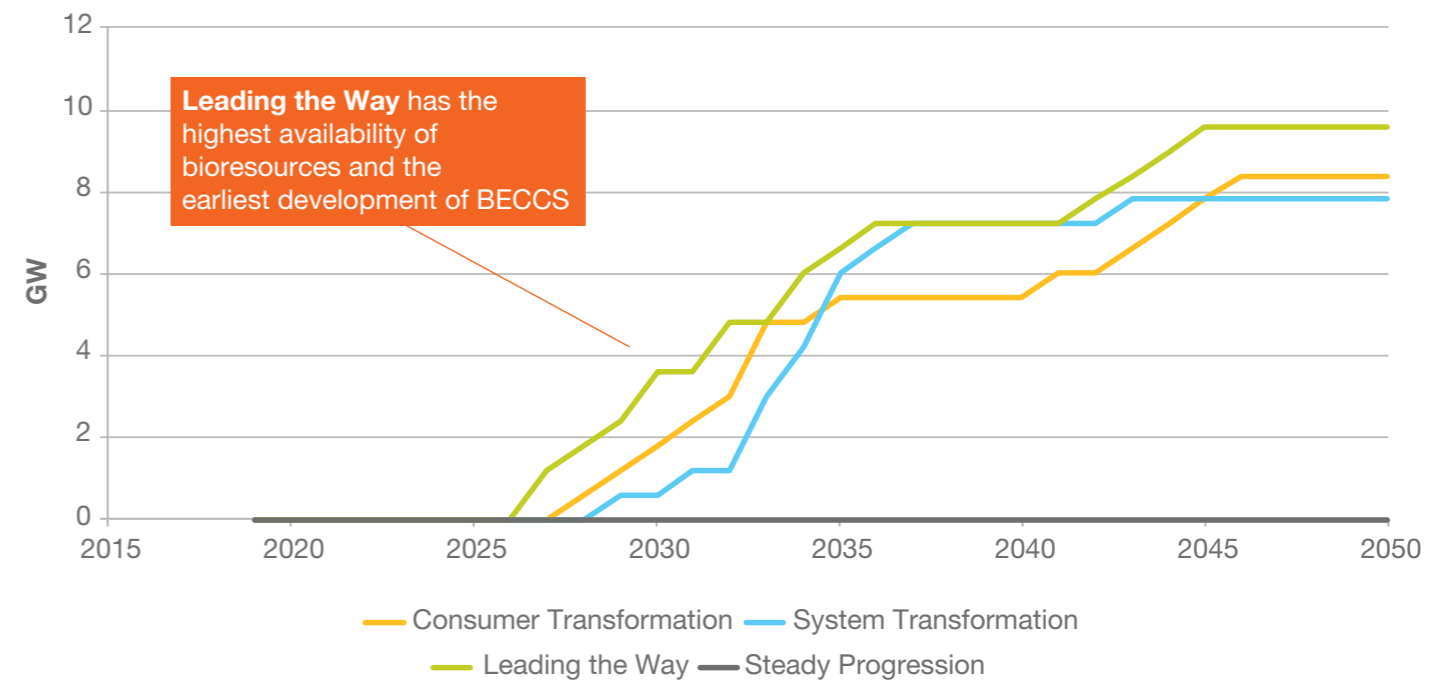
Figure SV.32: BECCS electricity generation capacity
