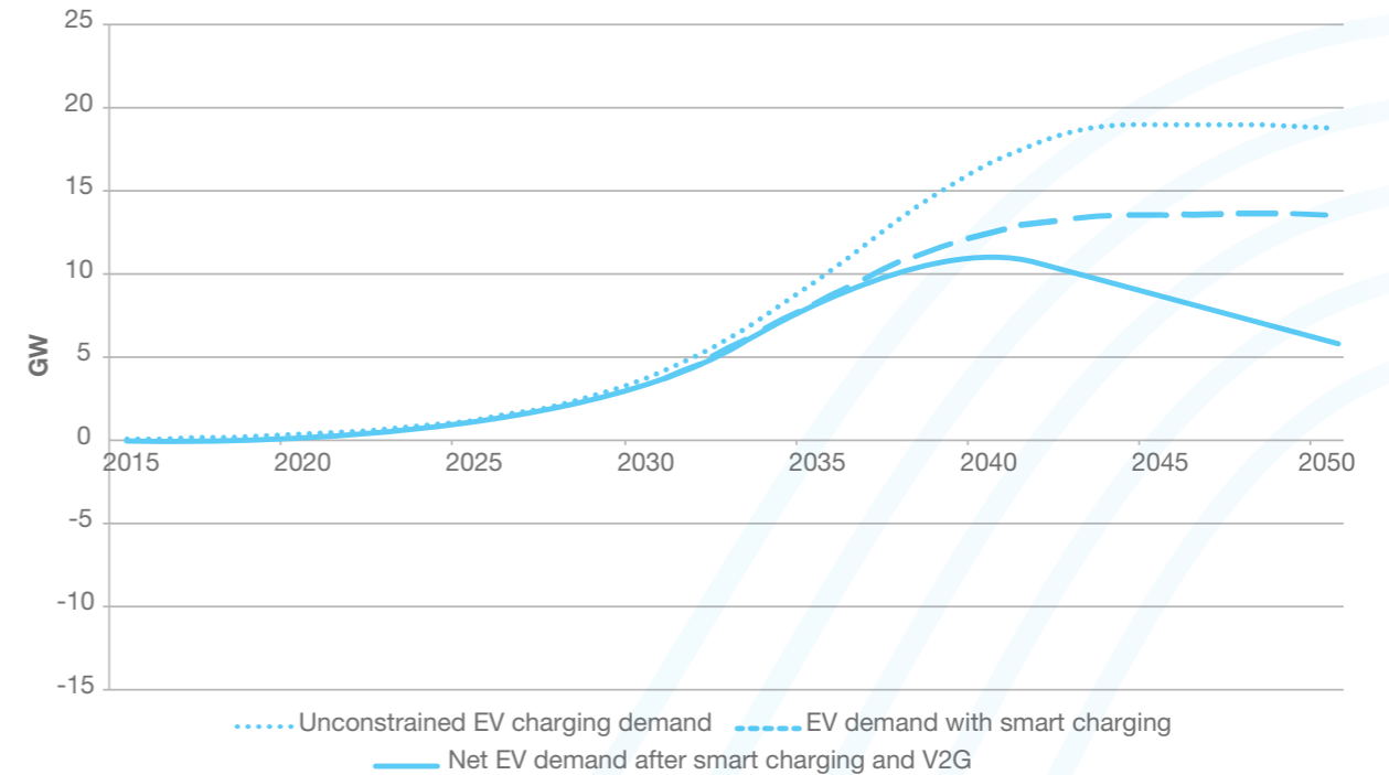
Figure SV.42: Electric vehicle charging behaviour at ACS 2 winter peak system demand
