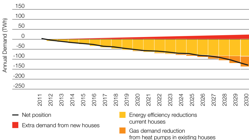
Figure 32. Changes in domestic gas demand: Gone Green
