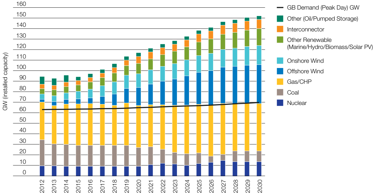
Figure 27. Demand and Generation Background: Gone Green
