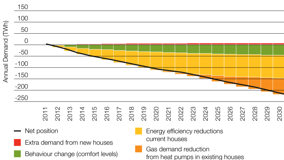
Figure 33. Changes in domestic gas demand: Accelerated Growth
