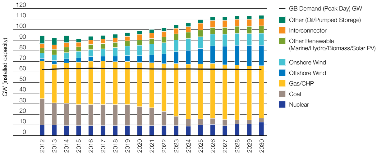
Figure 26. Demand and Generation Background: Slow Progression
