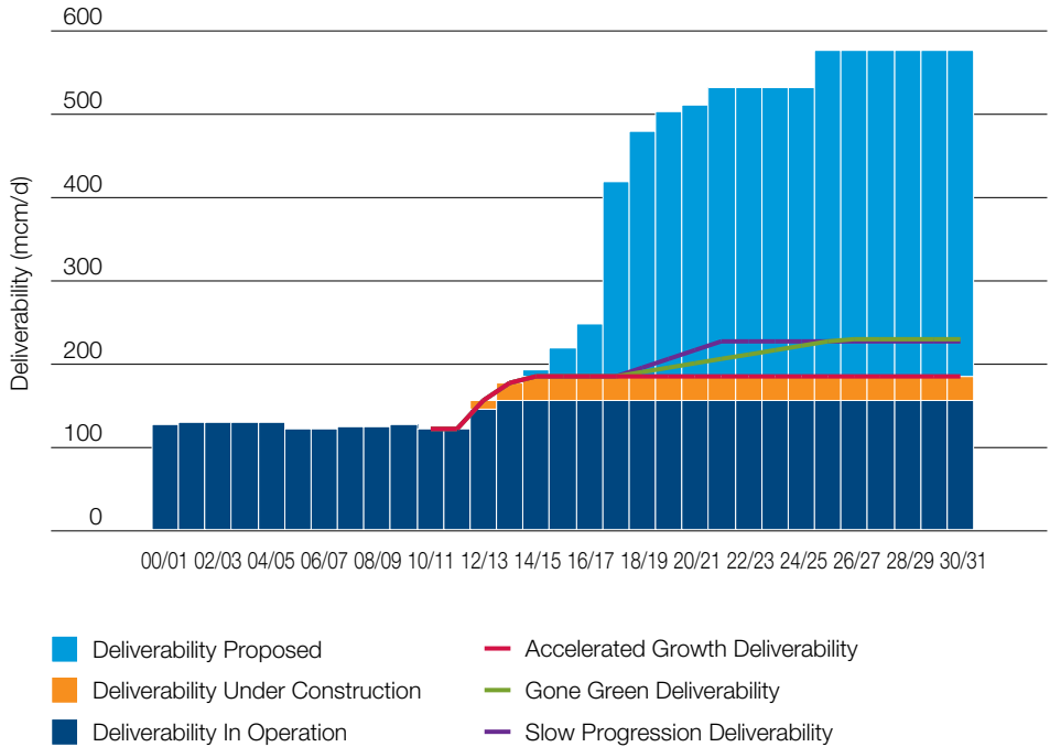
Figure 49. Storage Forecast (Deliverability)
