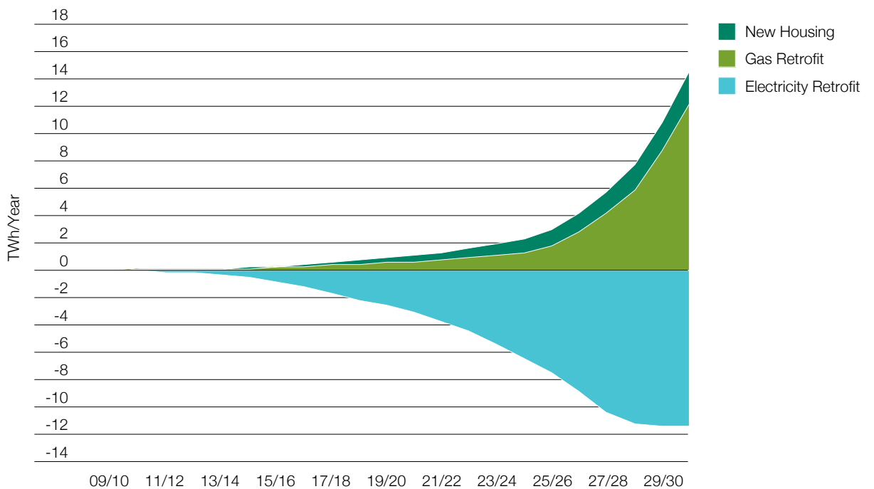
Figure 7. Changes in electricity demand due to domestic heat pumps: Gone Green
