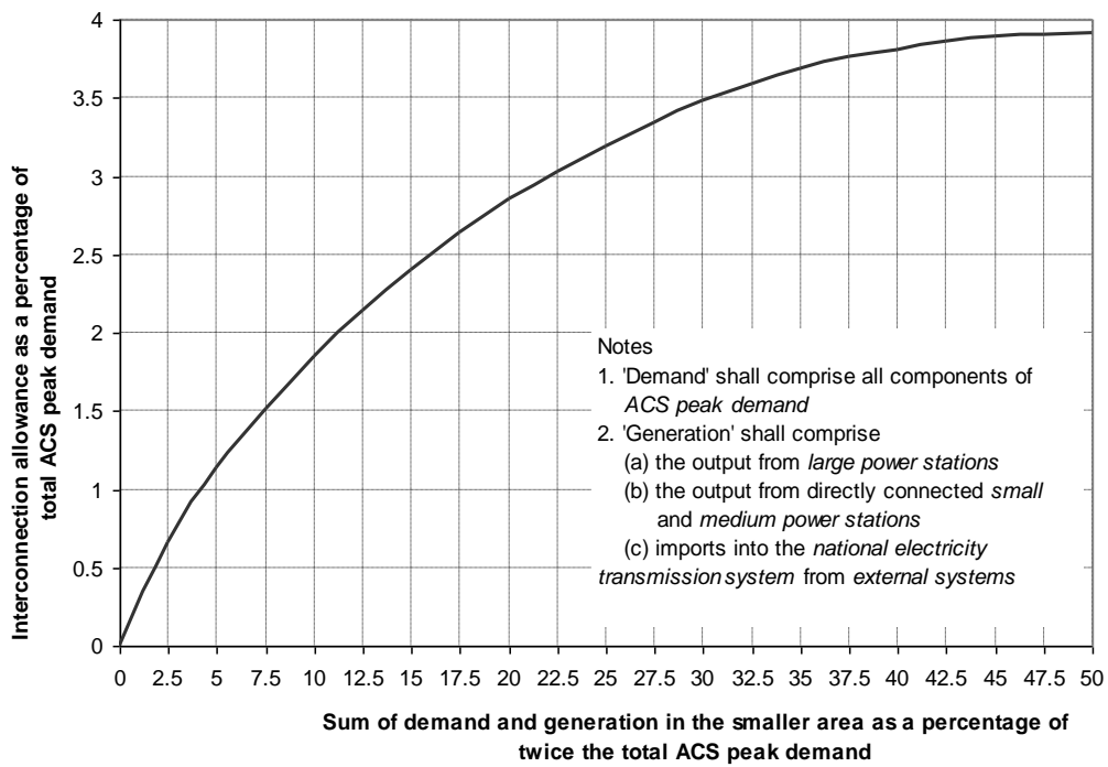
Figure D.1 Interconnection Allowance as a Function of Area Size (The 'Circle Diagram')
