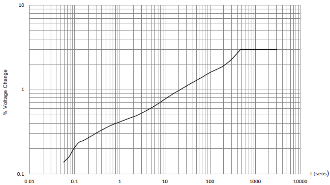
Figure 6.1 Maximum Voltage Step Changes Permitted for Operational Switching derived from ER EP P28 B.1.2
