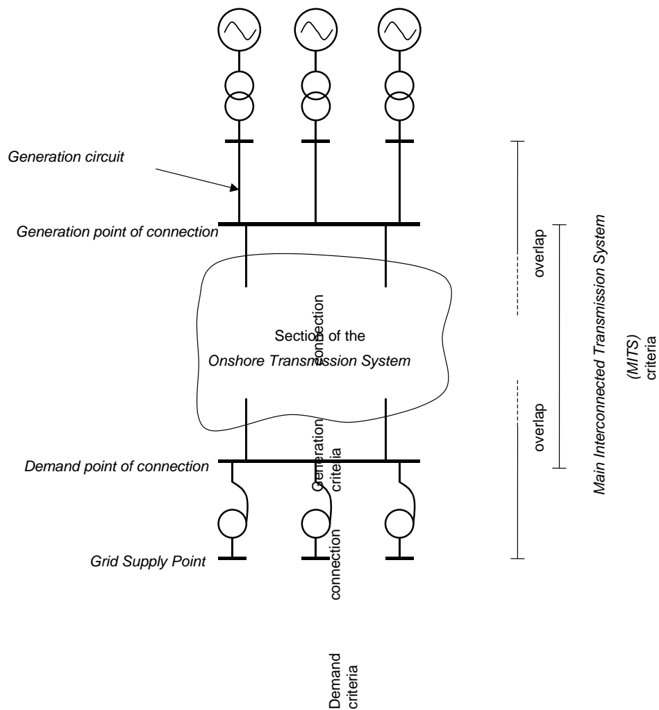
Figure 1.1 The onshore transmission system with a directly connected power station
