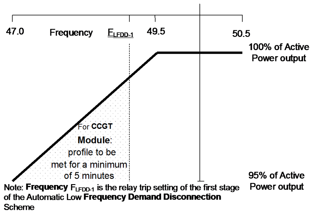
Figure ECC.6.3.3(a) Active Power Output with falling frequency for Power Generating Modules (including Electricity Storage Modules) and HVDC Systems when operating in an exporting mode of operation
