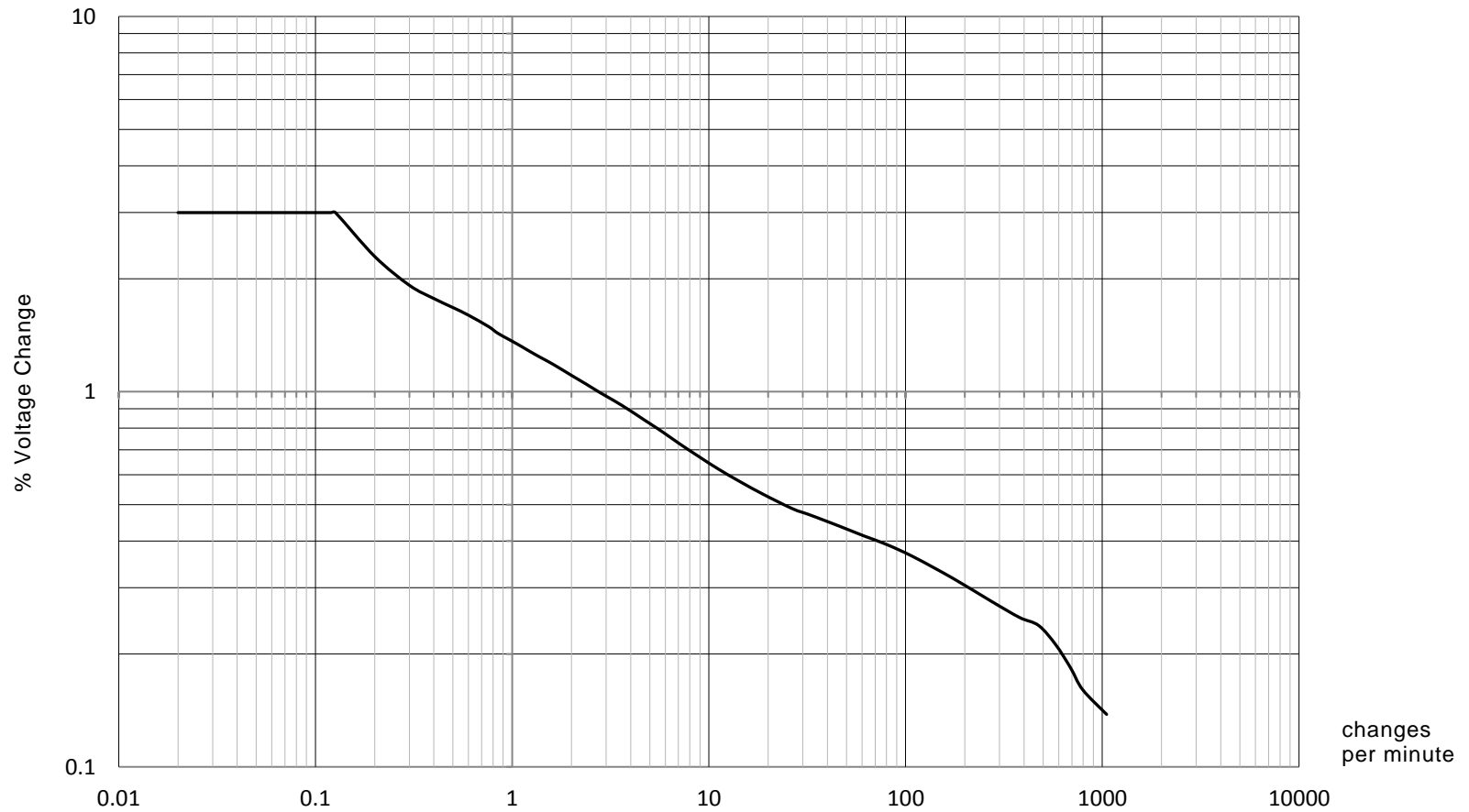
b) Maximum number of voltage changes per minute Figure B.1.2 — Pst = 0.5 curve for rectangular voltage changes
