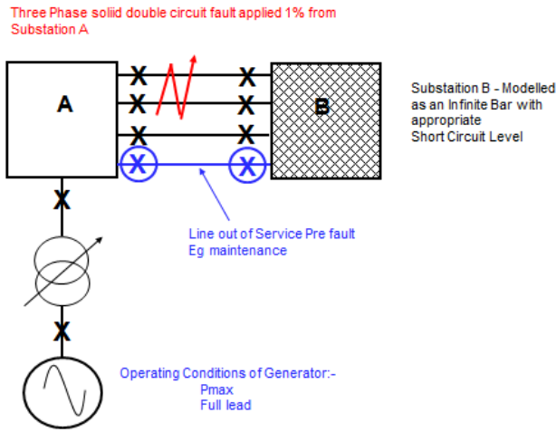
Figure 11.6(b) – Test Network Equivalent under Fault Conditions
