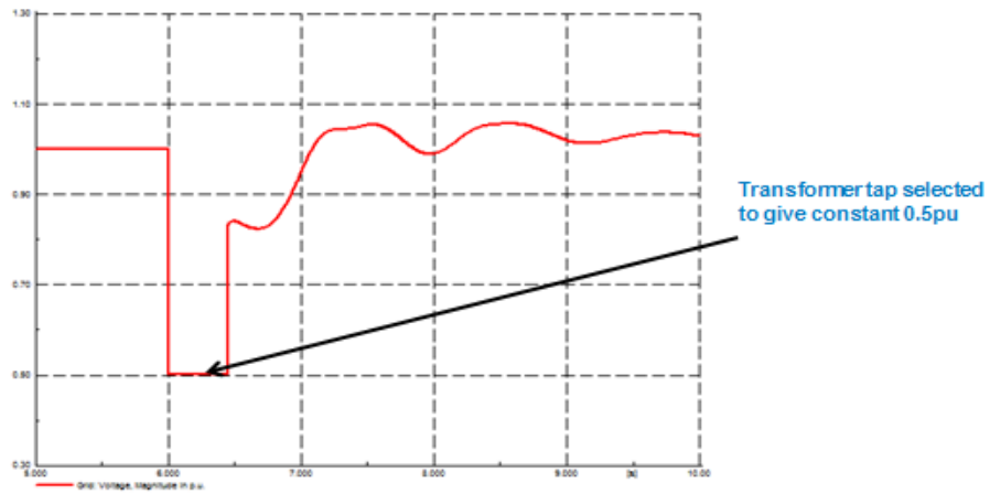
Figure 13.20 – Method 2 - Mode B Fault Ride Through Compliance – Method to obtain volt drop.
