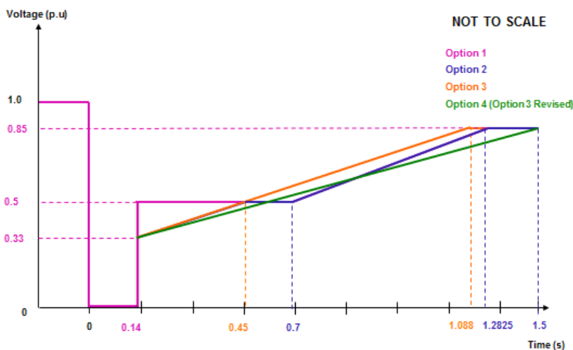
Figure 13.11 – Options Considered for Mode B Voltage Duration Curves based on initial studies.
