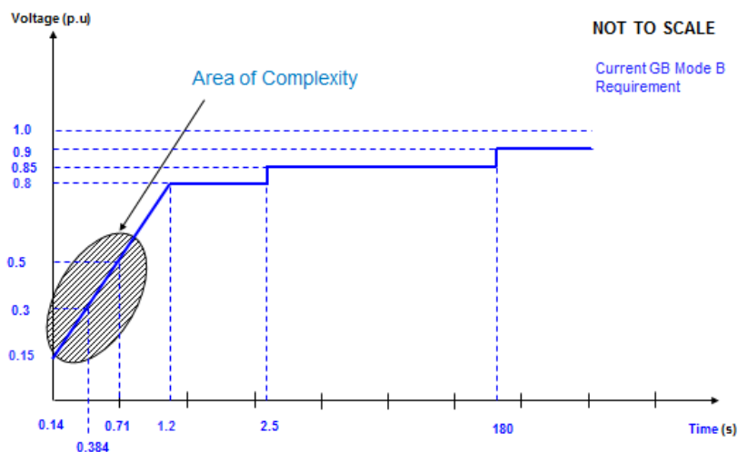
Figure 13.3 – GB Grid Code – Mode B Fault Ride Through Requirements – Area of Complexity
