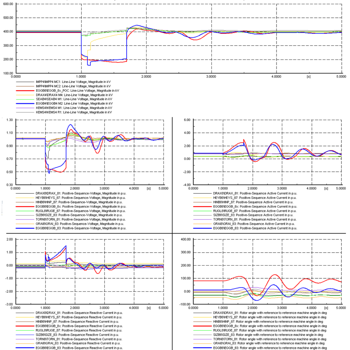
Figure A.44b Eggborough single M/C study (same as figure A.36a-e but with 30km of OHL).
