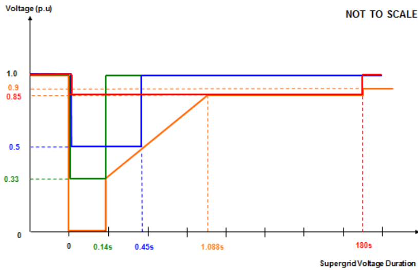
Figure 13.15 – Examples of Voltage dips as seen on the Transmission System superimposed on the proposed voltage against time curve.
