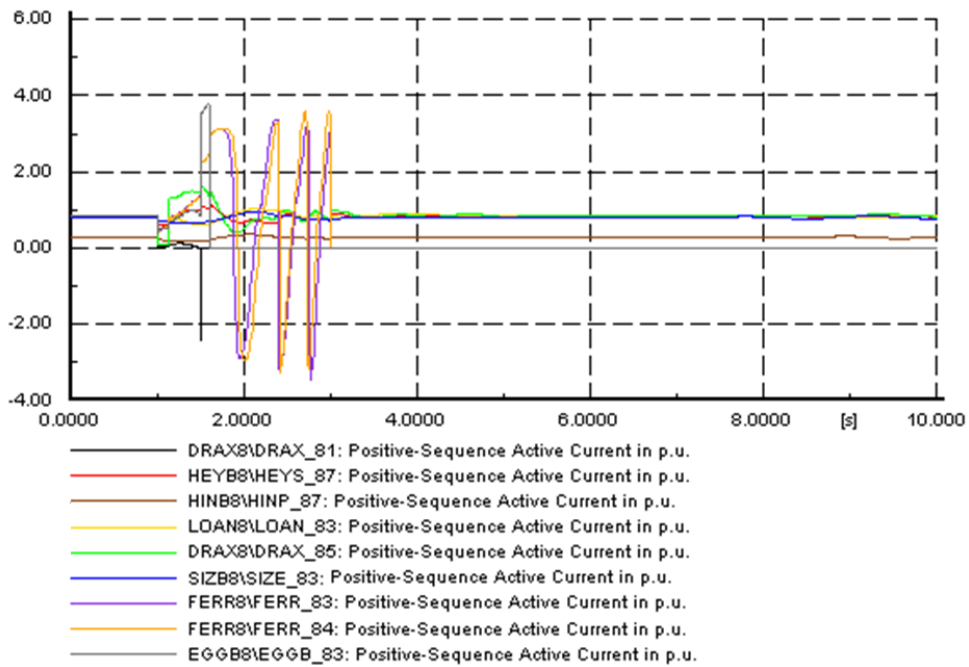
Figure A.26b – Active Current (i.e. Power at 1pu volts) as seen at generator terminals of various machines for more severe Eggborough / Drax study
