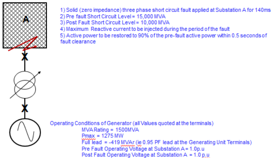
Figure 12.4 – Parameters and model issued by NGET for the Generator to undertake Mode A (RfG Compliant) Fault Ride Through Compliance Studies
