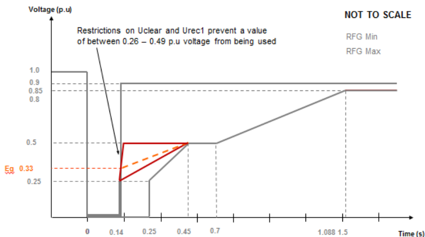
Figure 10.5 – Limitations on voltage against time curves
