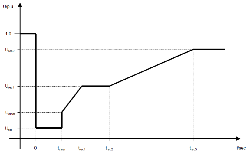
Figure 8.7 – Voltage Against Time Curve – Reproduction of RfG Fig 3
