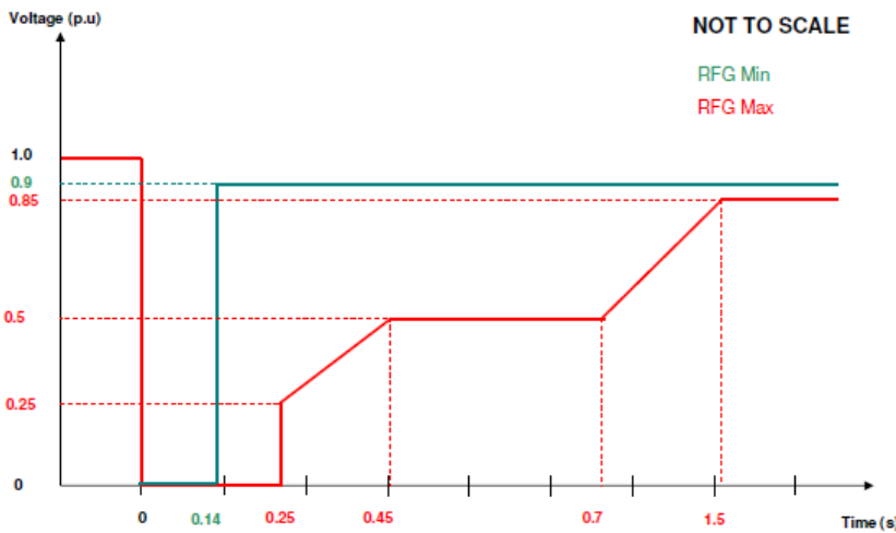
Figure 10.3 – Range of RfG Voltage Against Time Parameters
