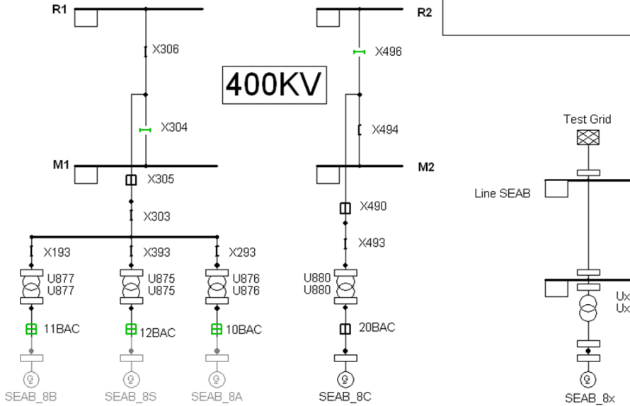
Figure A.32 – Seabank single machine model SEAB_8x compared simultaneously with SEAB_8C connected to GB system
