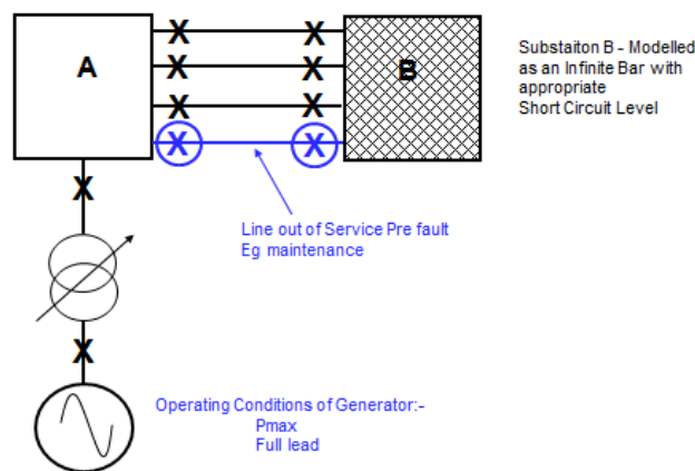
Figure 11.6(a) – Pre Fault Test Network Equivalent
