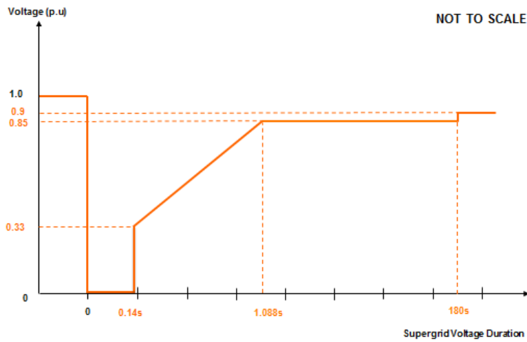
Figure 13.13(a) – Final Proposed Mode B Voltage Duration Curve.
