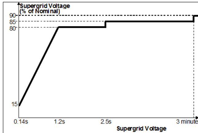
Figure 13.1 – Current GB Grid Code Mode B Voltage Duration Curve Fault Ride Through Requirements
