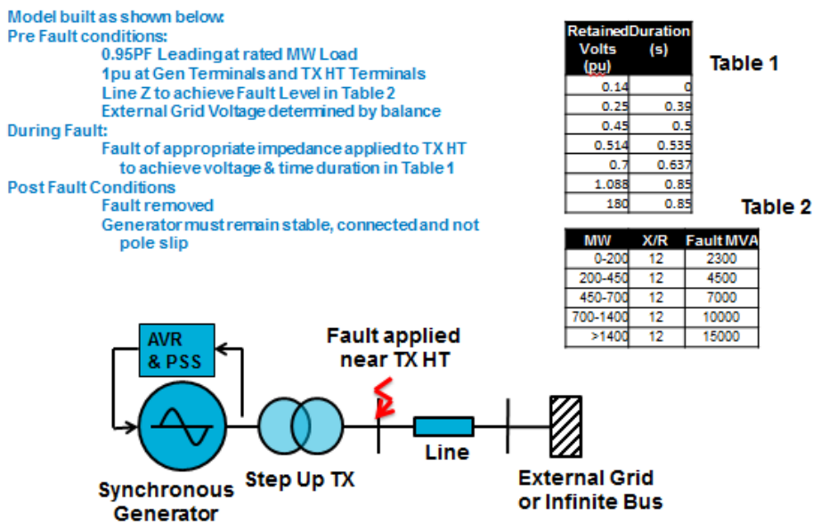
Figure 13.17 – Method 1 – demonstration of Mode B Fault Ride Through compliance
