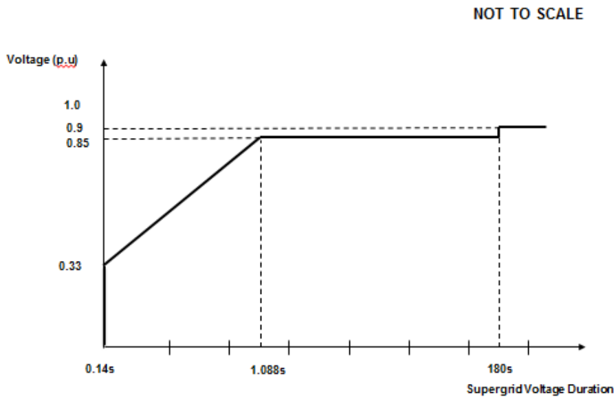
Figure 13.13(b) – Final Proposed Mode B Voltage Duration Curve.
