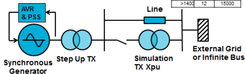
Figure 13.19 – Method 2 – demonstration of Mode B Fault Ride Through compliance
