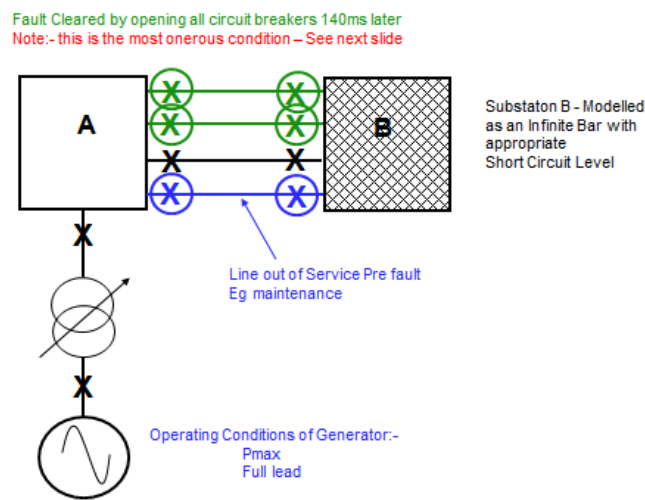
Figure 11.6(c) – Post Fault Network as an Equivalent
