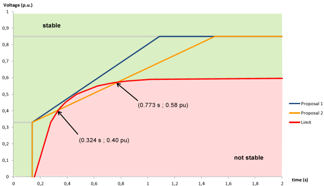
Figure 13.12 – Critical Fault Clearing Times for a 1780 MW Generator against proposed Mode B voltage duration curve.
