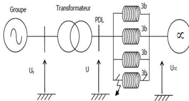
Figure 11.7 – RTE to Modelling Low Voltage Fault Ride Through
