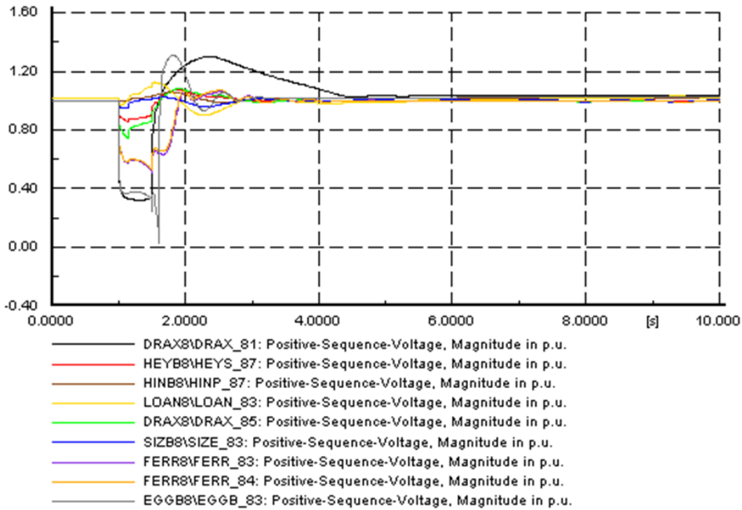
Figure A.31a – Voltage profile as seen at generator terminals of various machines for more severe single circuit Eggborough / Drax study
