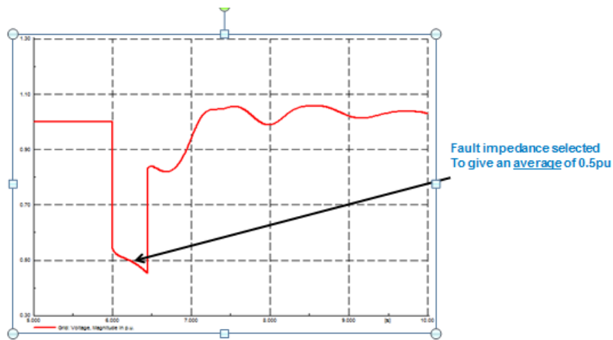
Figure 13.18 – Method 1 - Mode B Fault Ride Through Compliance – Method to obtain an average volt drop.
