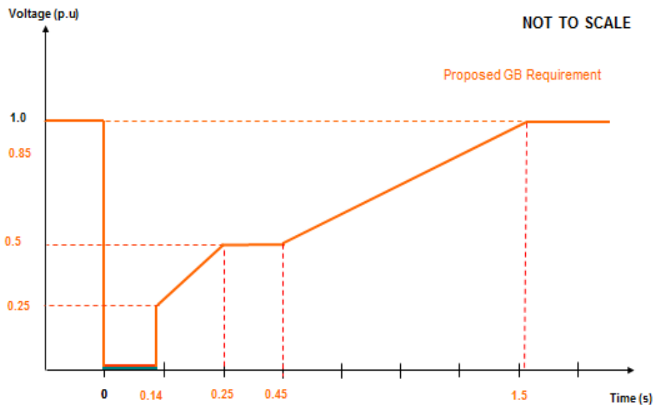
Figure 10.15 – Proposed GB Voltage against time curve for the Fault Ride Through Capability of a Synchronous Generating Unit connected at Supergrid Voltage
