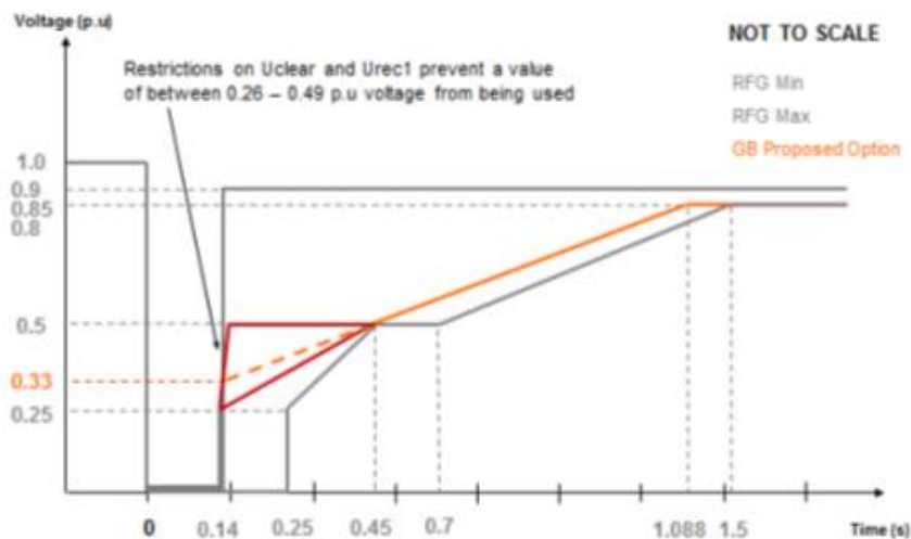
Figure A2.31 – Limitations on voltage against time curves
