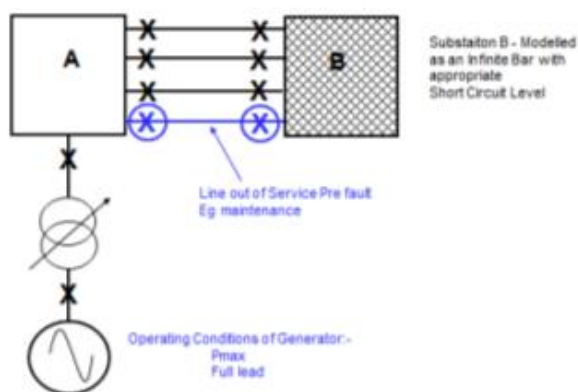
Figure A2.49(a) – Pre Fault Test Network Equivalent
