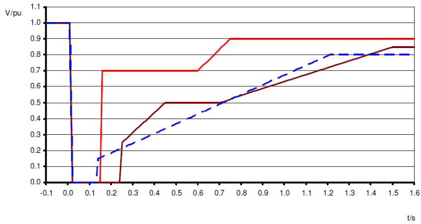
Fault Ride Through - Transmission Connected Synchronous Generator
