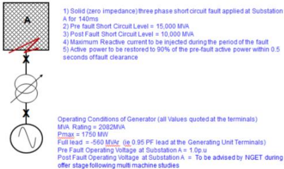
Figure A2.58 – Parameters and model issued by NGET for the Generator to undertake Mode A (RfG Compliant) Fault Ride Through Compliance Studies
