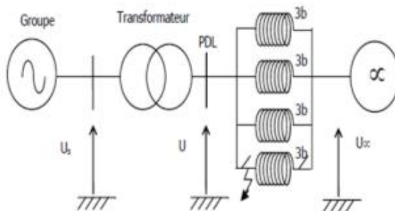
Figure A2.50 – RTE to Modelling Low Voltage Fault Ride Through
