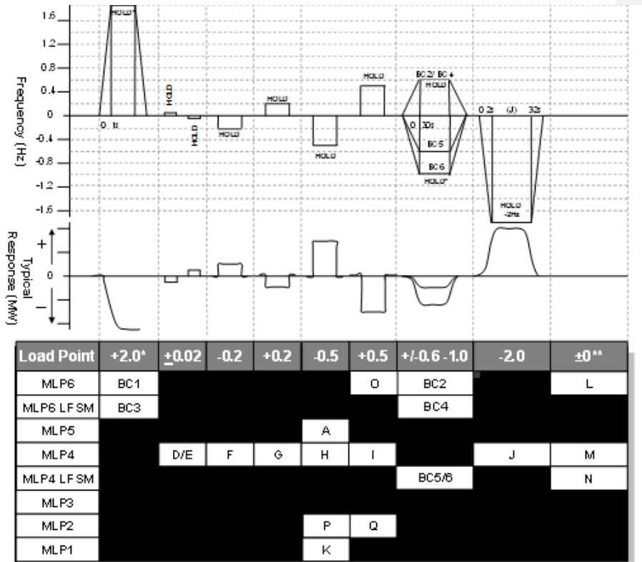
Figure 2: Frequency Response Capability LFSM-O, LFSM-U and FSM Step Response Tests
