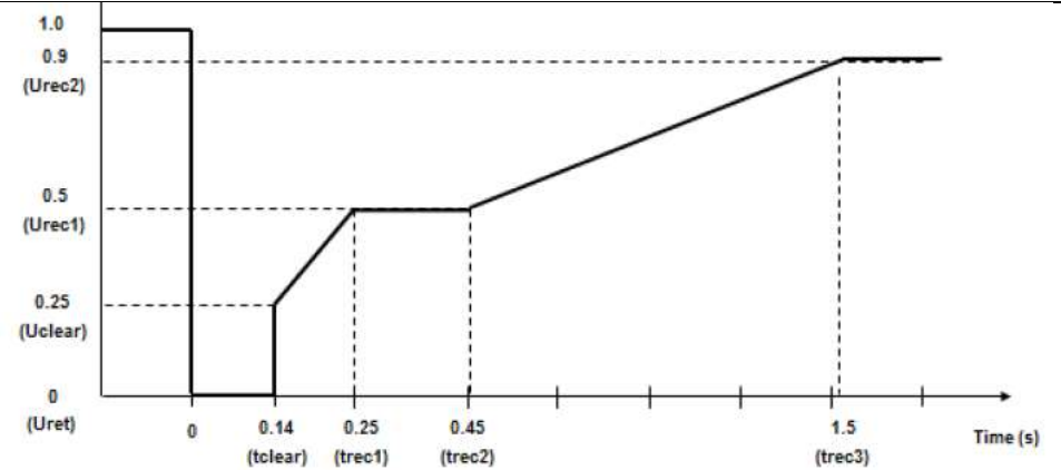
Figure ECC.6.3.15.4 - Voltage against time curve applicable to Type D Sync
