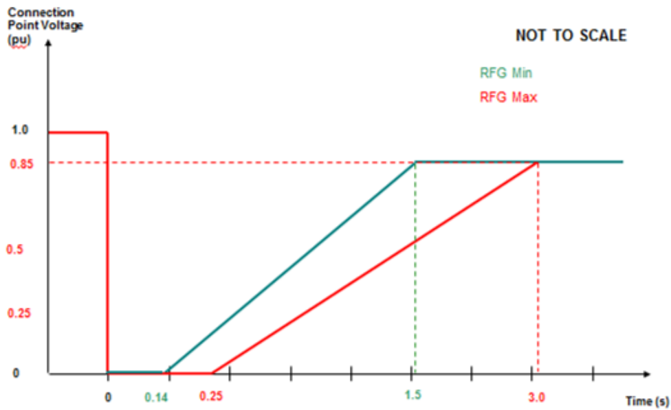
Figure 3.9 – Range of voltage against time parameters for Type D Power Park Modules connected at or above 110kV
