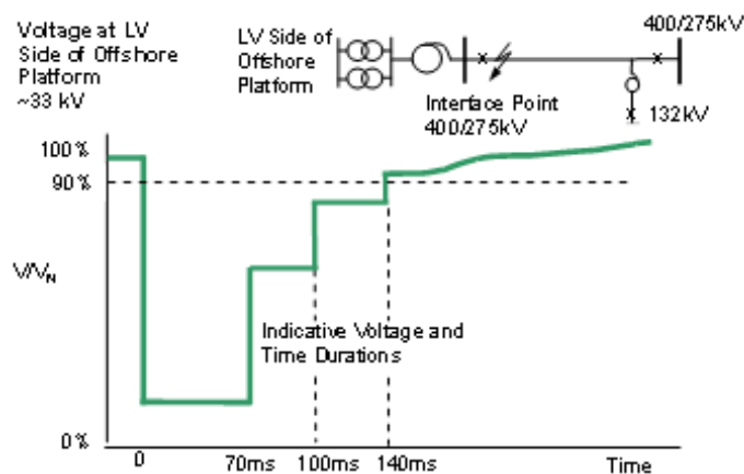
Typical fault cleared in 140ms:- 3 ended circuit
