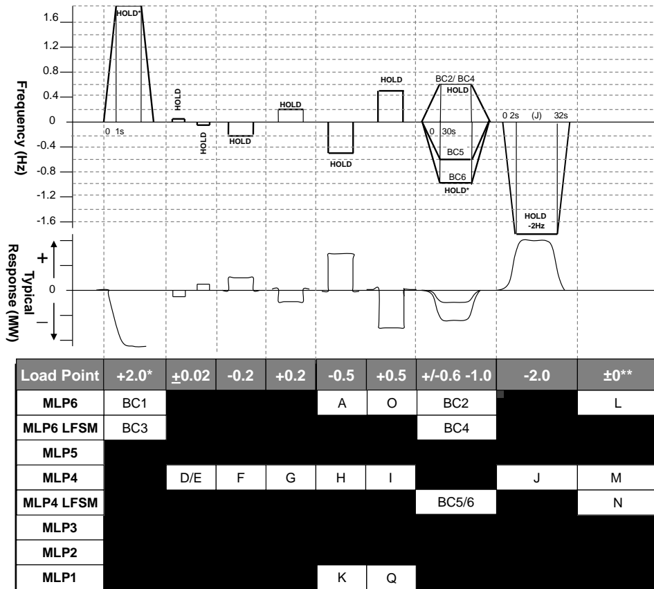
ECP.A.7.5. Figure 2 – Frequency Response Capability LFSM-O, LFSM-U, FSM Step R System islanding and step response tests
