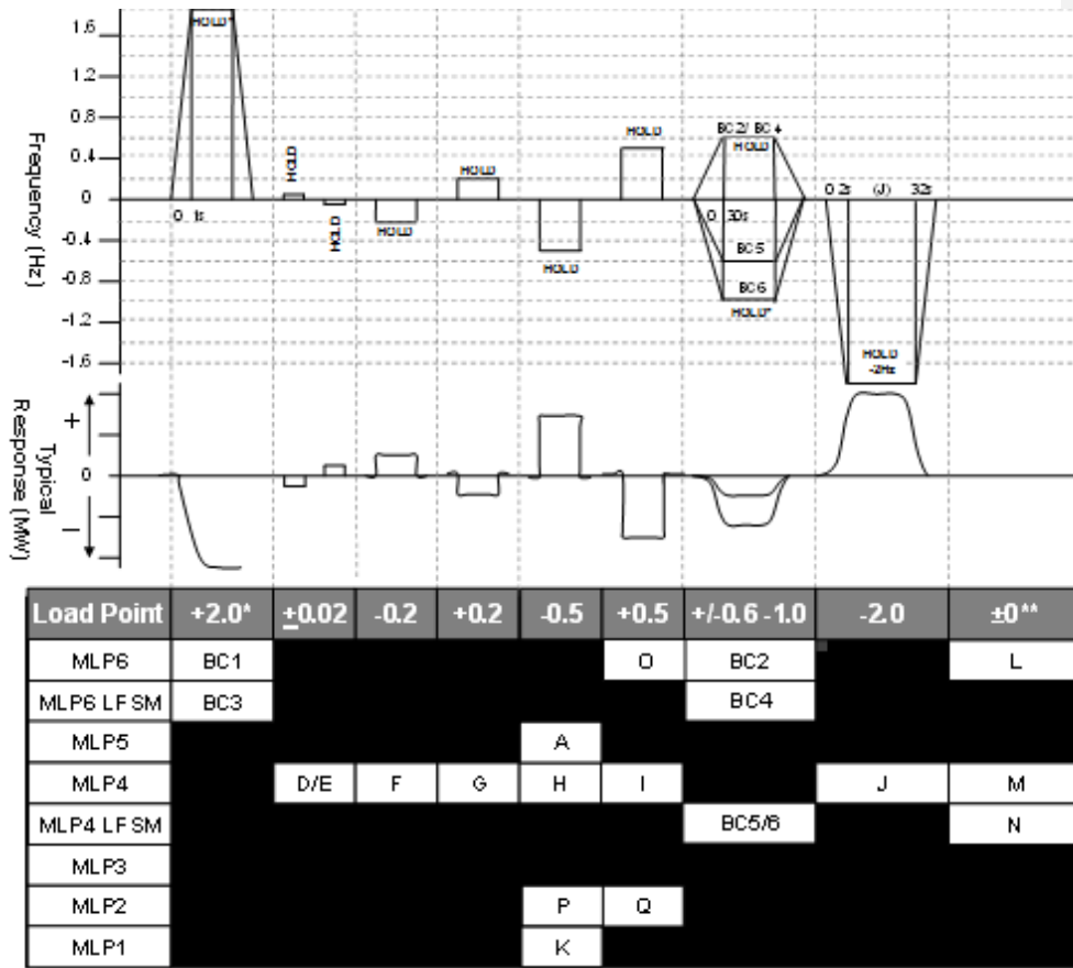
Figure 2: Frequency Response Capability LFSM-O, LFSM-U and FSM Step Response Tests System islanding and step response tests
