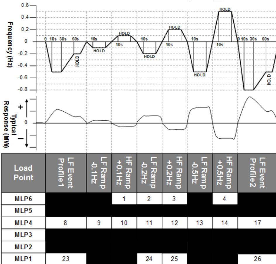
ECP.A.7.5. Figure 1 – Frequency R esponse Capability FSM Ramp Response volume tests
