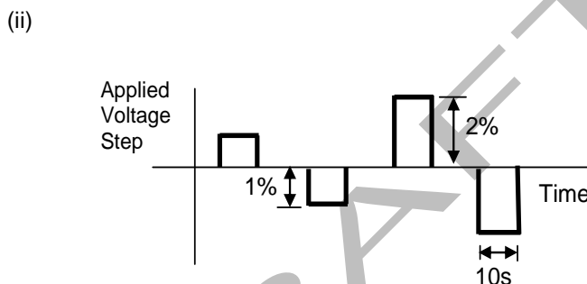
ECP.A.6.5 Figure 2 – Step injection sequence for voltage control tests
