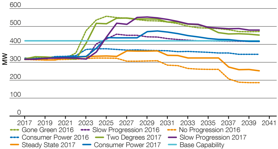
Figure B3b.2 Required transfer and base capability for boundary B3b
