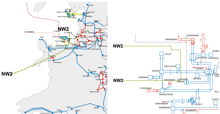
Figure NW2.1 Geographic and single-line representation of boundary NW2
