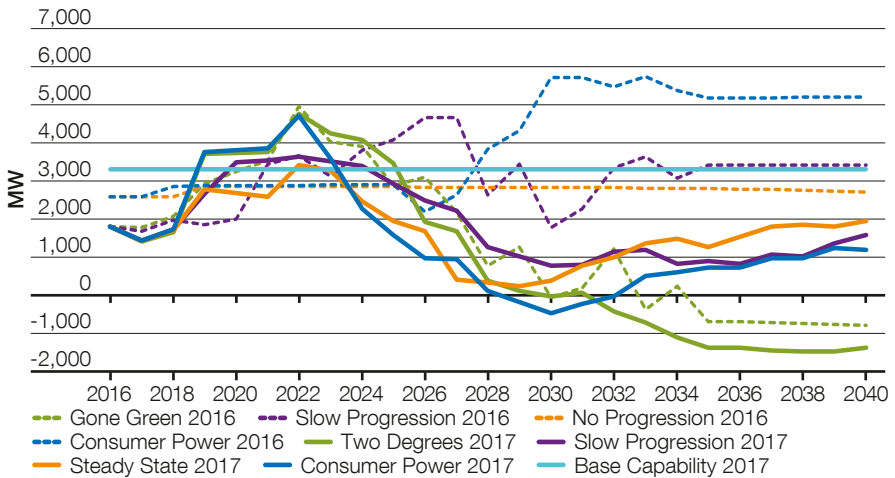
Figure SC2.2 Required transfer and base capability for boundary SC2
