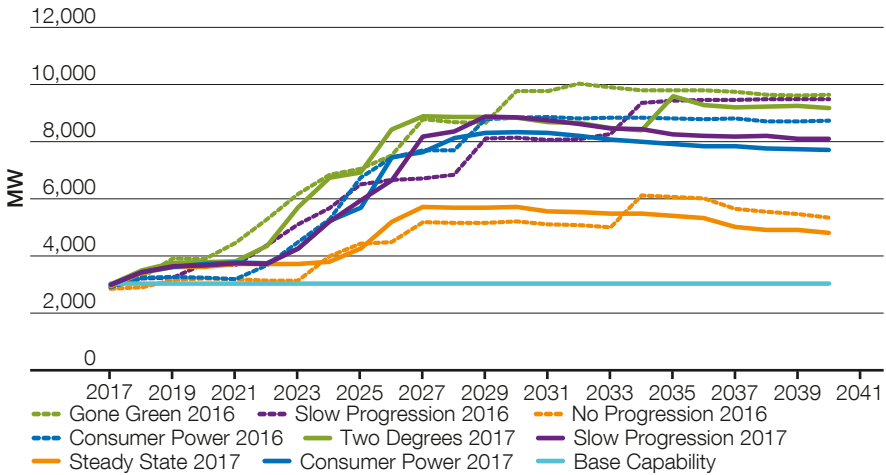
Figure B4.2 Required transfer and base capability for boundary B4
