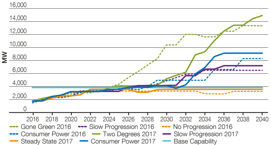
Figure EC5.2 Boundary export requirements and base capability for boundary EC5
