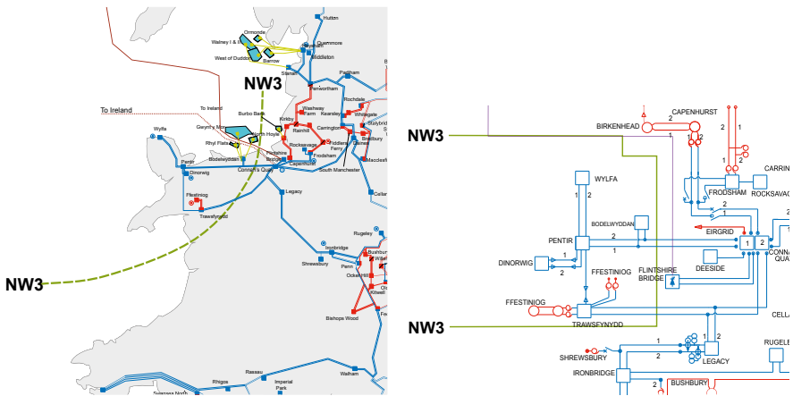
Figure NW3.1 Geographic and single-line representation of boundary NW3
